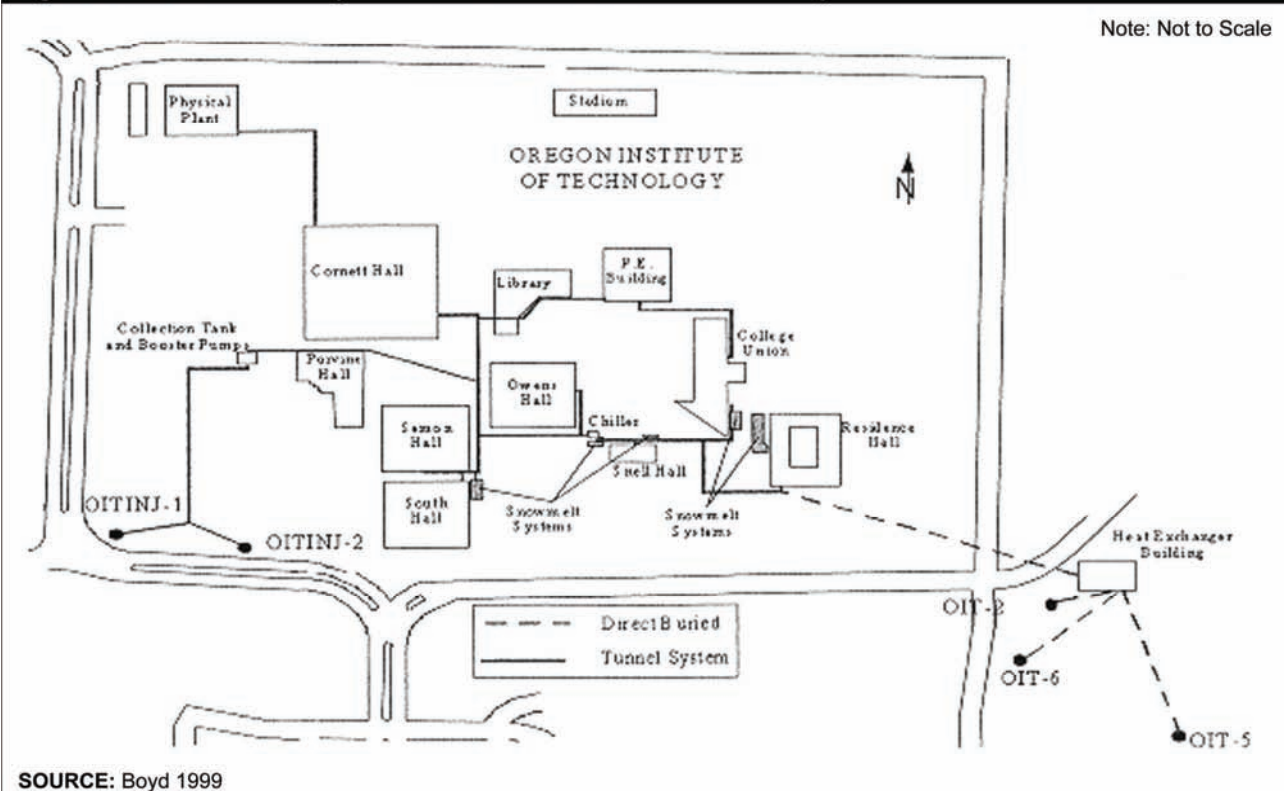
Figure 2.3-1: General Layout of the Current OIT Geothermal System
