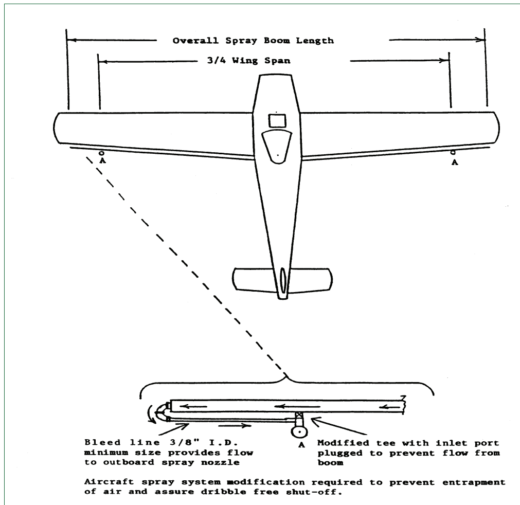
Figure L-1 Diagram of Spray Boom Flow Through Bleed Line to Outermost Nozzles
