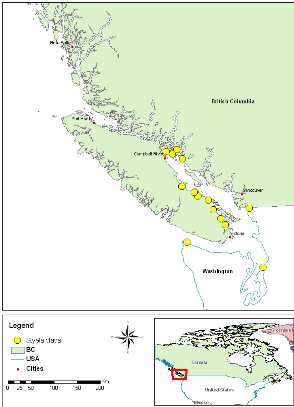
Figure 5: Distribution of Styela clava in Pacific Canada based on reference records, aquaculture site surveys and collector plate settlement experiments by DFO.
