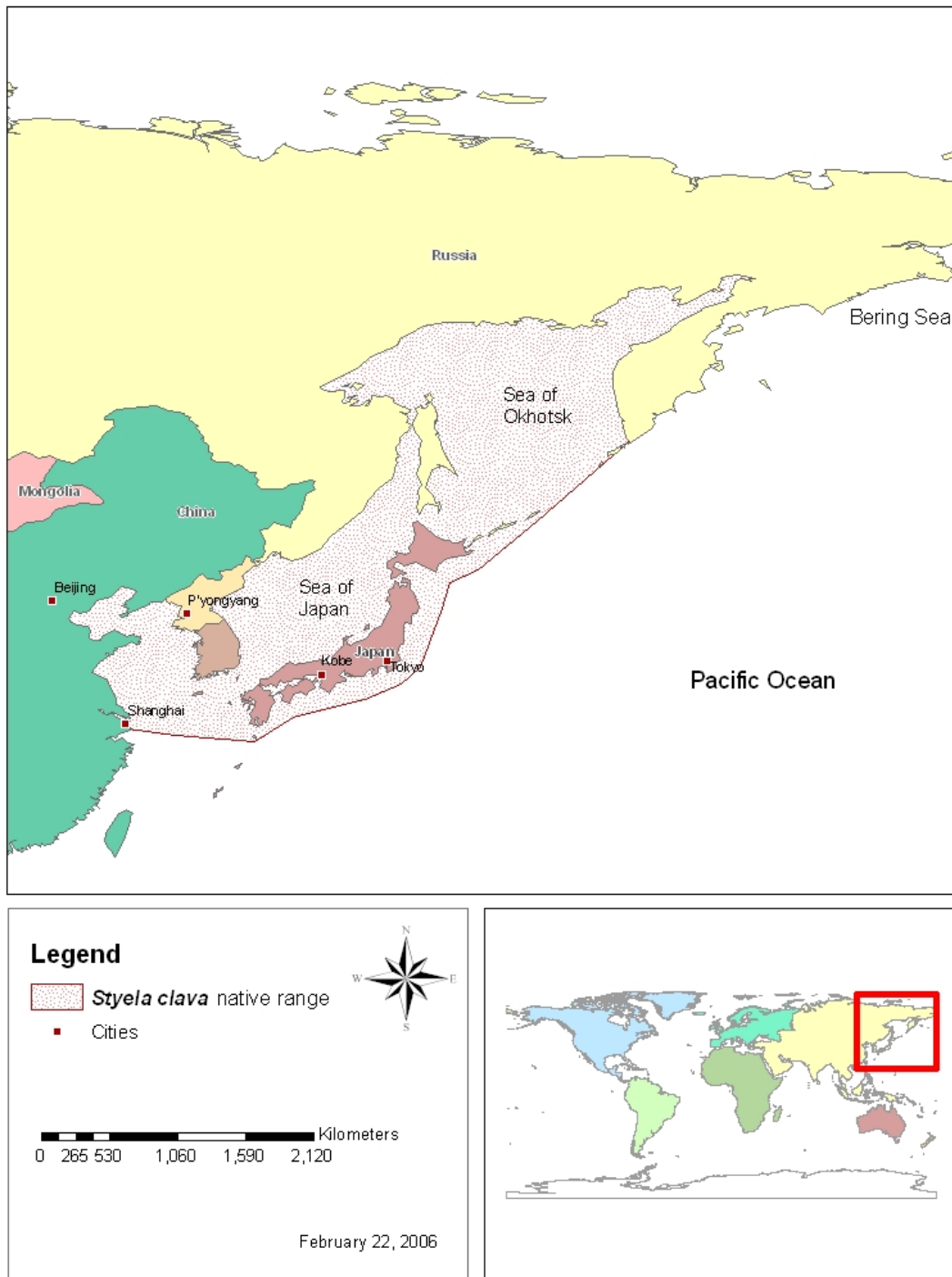
Figure 3: Northwest Pacific, native range of the ascidian Styela clava . Inset map shows extent of map on world continents.
