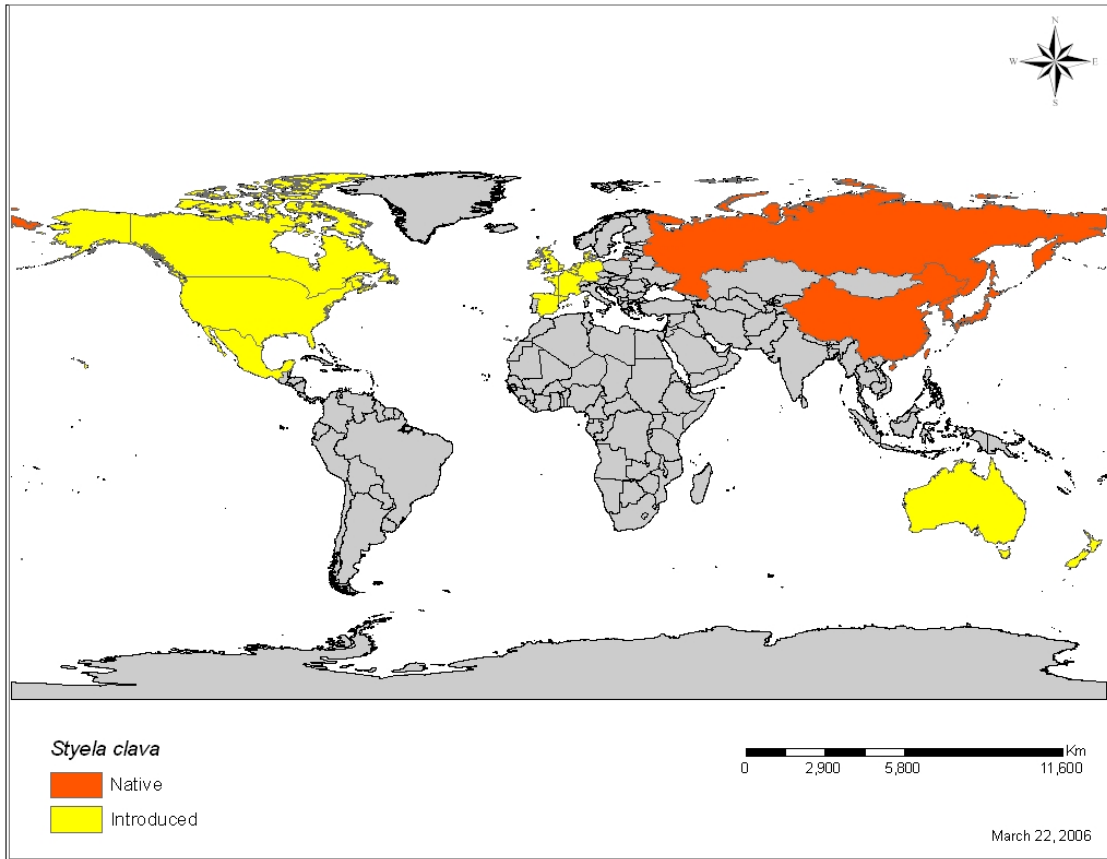
Figure 4: Countries where Styela clava occurs worldwide: the native range is in red and introduced in yellow. Styela clava is not necessarily found over the entire coast line of those countries highlighted.
