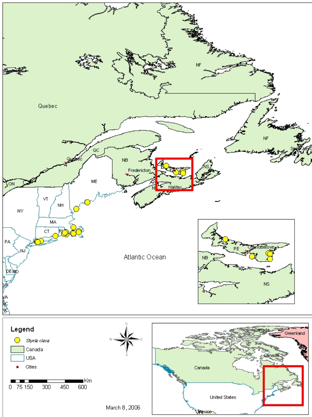
Figure 6: Distribution of Styela clava on the east coast of North America. Small inset map shows distribution on Prince Edward Island. Large inset map shows reference box within Canada.
