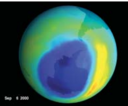
TOMS image of largest-ever ozone hole over Antarctica.
