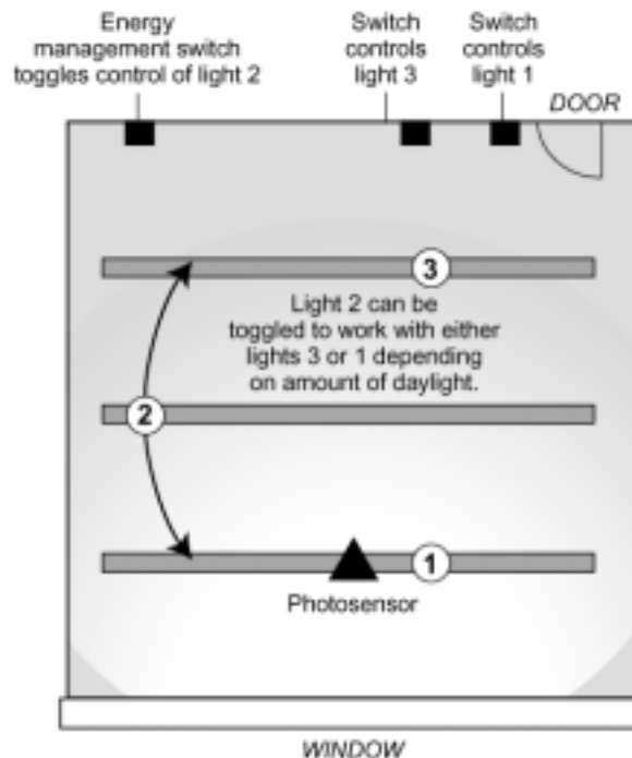
Figure 22 – Simple Windowed Classroom Control
