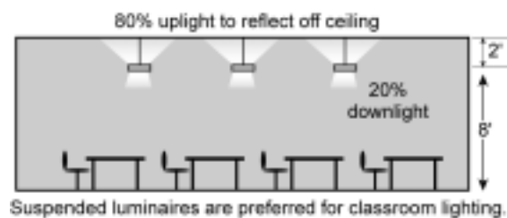
Figure 15 – Recessed vs. Suspended Luminaires
