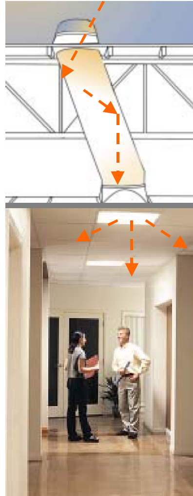
Tubular skylights work well for small spaces, such as toilet rooms, locker rooms, kitchens, and interior corridors.
