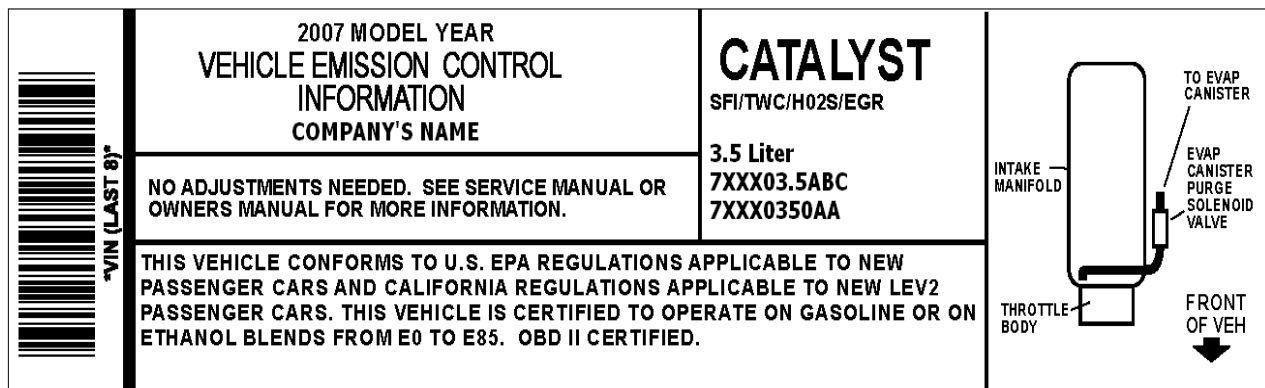
Figure 2 Example Emission Label for Some 2007 and Earlier Model Year Vehicles
