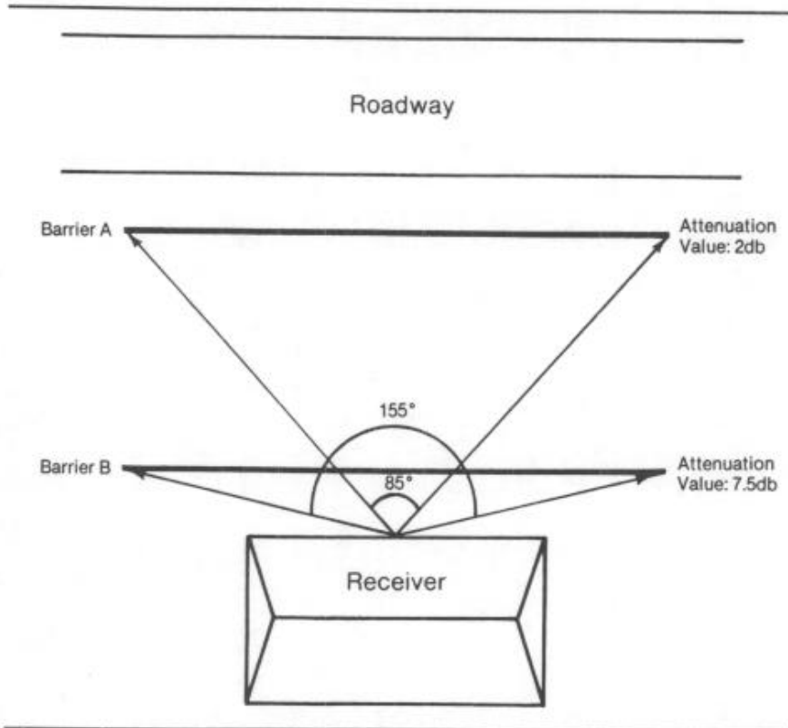
Figure 9 Effect of Moving Barrier Closer to Receiver
