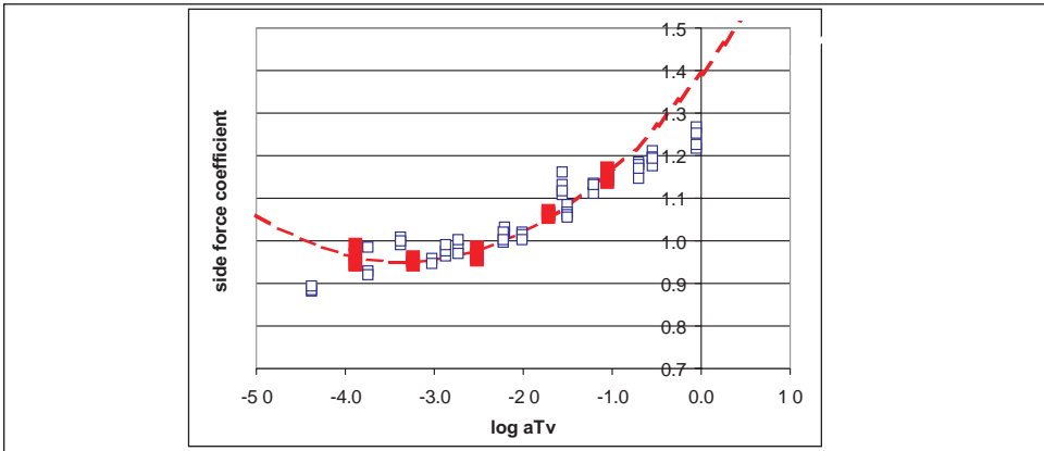
Figure 11.44: Side force coefficient of compound A (an OE-SBR black filled tire tread compound) on wet blunt alumina 180 as a function of \log a_T v obtained at three speeds and five temperatures (open squares) with a quadratic equation fitted to the data (black solid line). The red marked points were obtained at one speed for five temperatures with the dotted red line the best-fit quadratic equation, showing the risk of extrapolating from a limited set of data.
