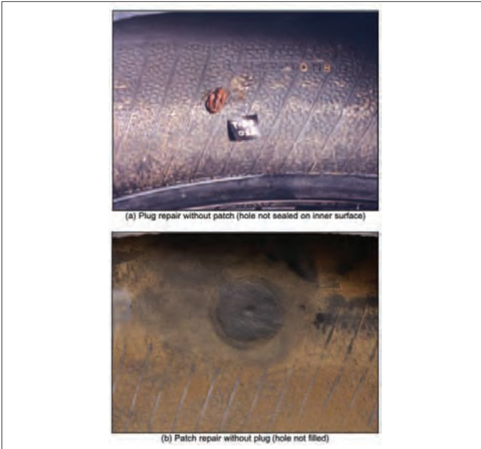
Figure 15.19: Examples of improper puncture repair
