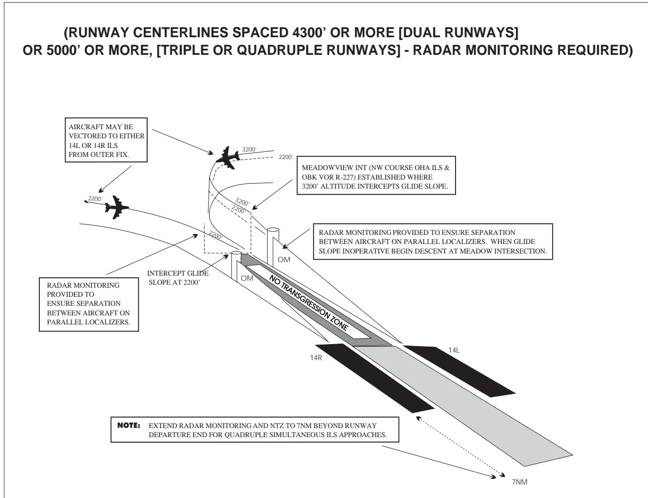
FIG 5-4-20 Simultaneous Parallel ILS Approaches
