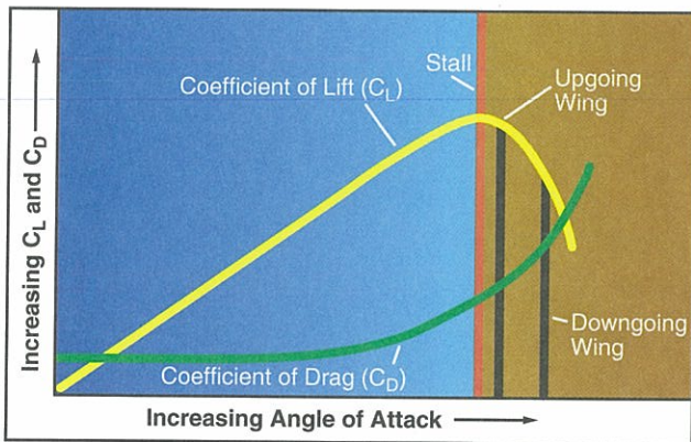
Figure 3-27. This graph depicts the relative coefficients of lift and drag for each wing during a spin. Note that the ascending wing experiences more lift and less drag. The opposite wing is forced down and back due to less lift and increased drag.
