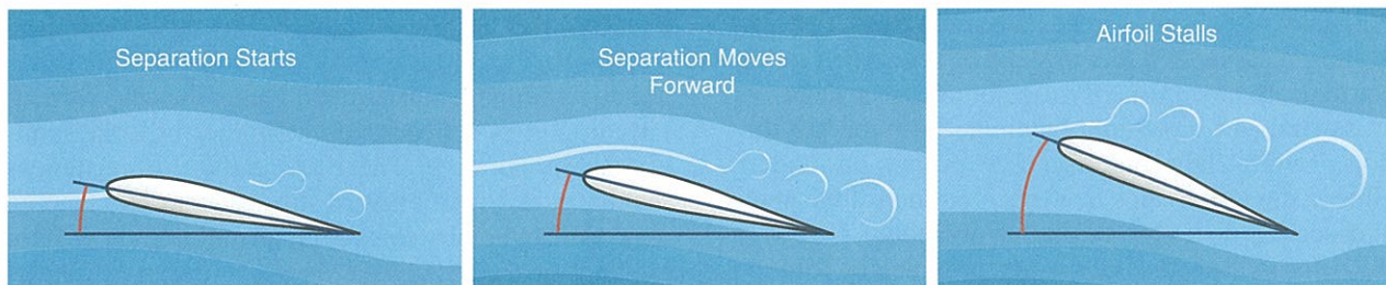
Figure 3-25. Increasing the pitch attitude beyond the critical angle of attack or C_{Lmax} causes progressive disruption of the airflow from the upper surface of the wing. At first the airflow begins to separate at the trailing edge. As the angle of attack is further increased, the airflow separation progresses forward until the wing is fully stalled.
