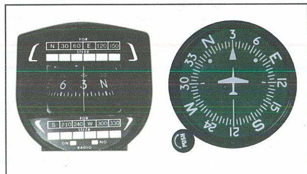
Figure 4-26. Setting the heading indicator.
