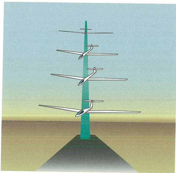
Figure 7-33. Forward slip.
