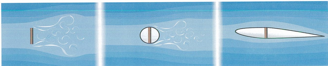
Figure 3-9. Streamlined airfoil designs greatly reduce form drag by reducing the amount of airflow separation.
