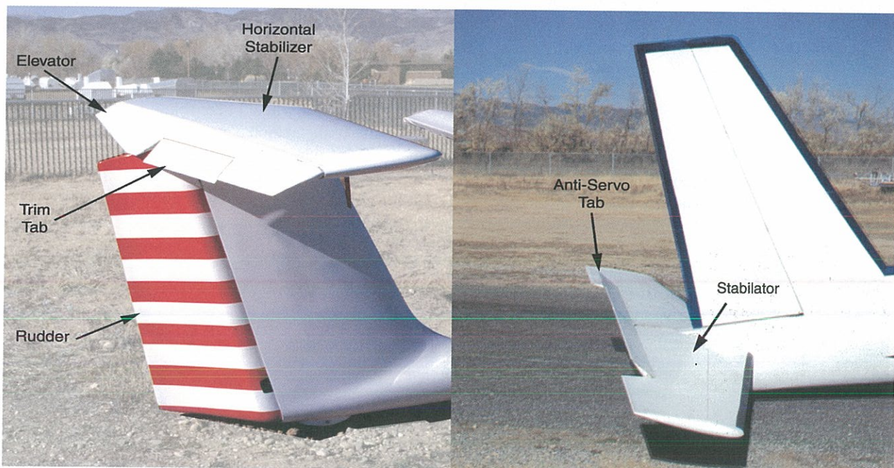
Figure 2-5. Empennage components and trim tabs.
