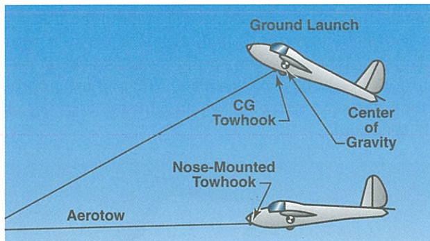
Figure 2-6. Towhook locations.
