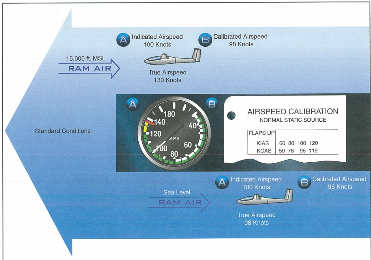
Figure 4-2. The three types of airspeed you should know include calibrated airspeed, indicated airspeed, and true airspeed.
