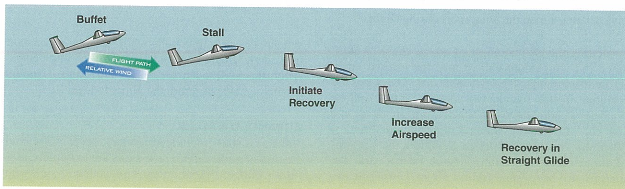
Figure 7-29. Stall recovery.
