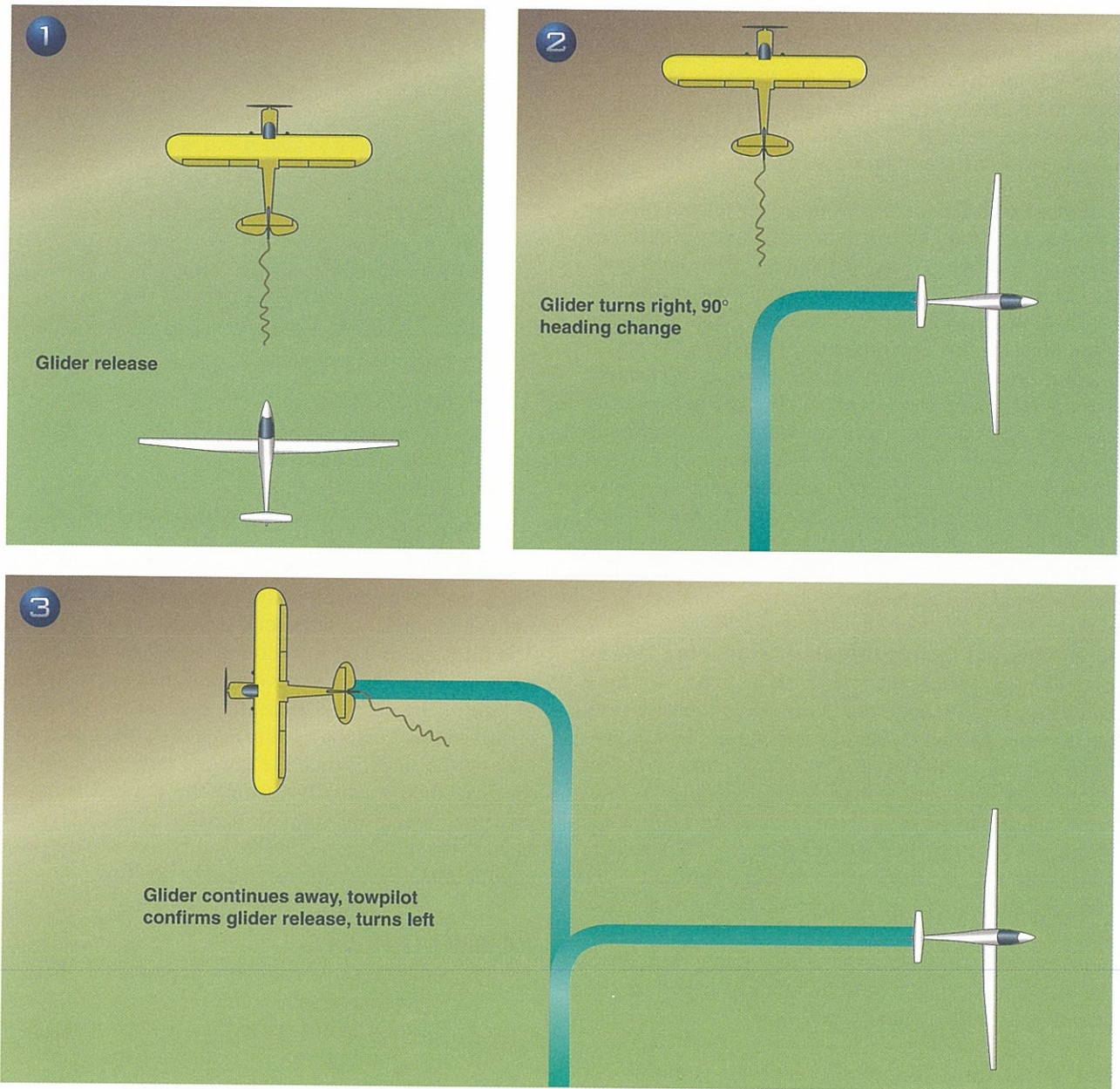
Figure 7-10. Aerotow release.
