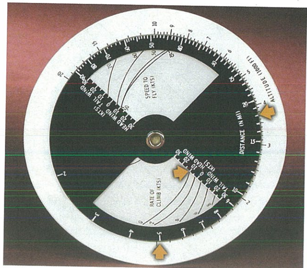
Figure 11-3. Circular glide calculator.
