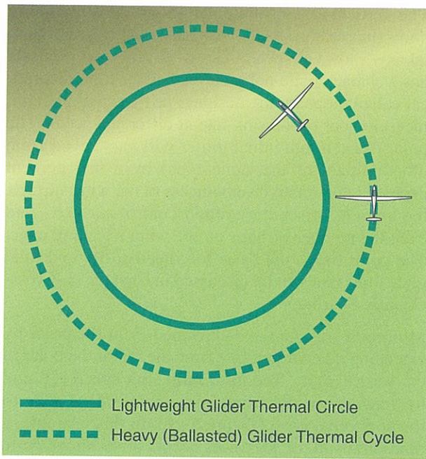
Figure 5-6. Effect and added weight on thermaling turn radius.
