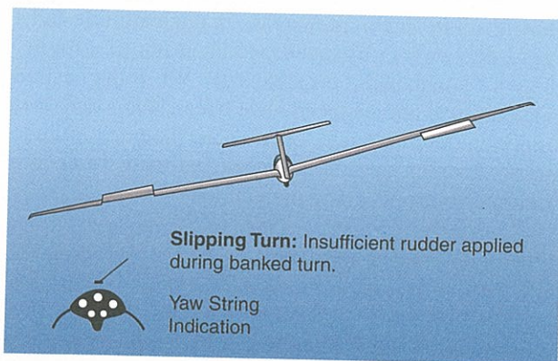
Figure 7-26. Slipping turn.
