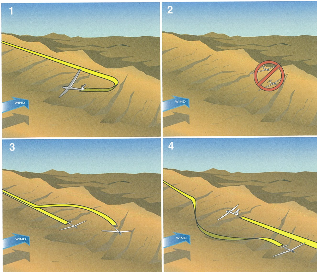
Figure 10-15. Ridge rules.
