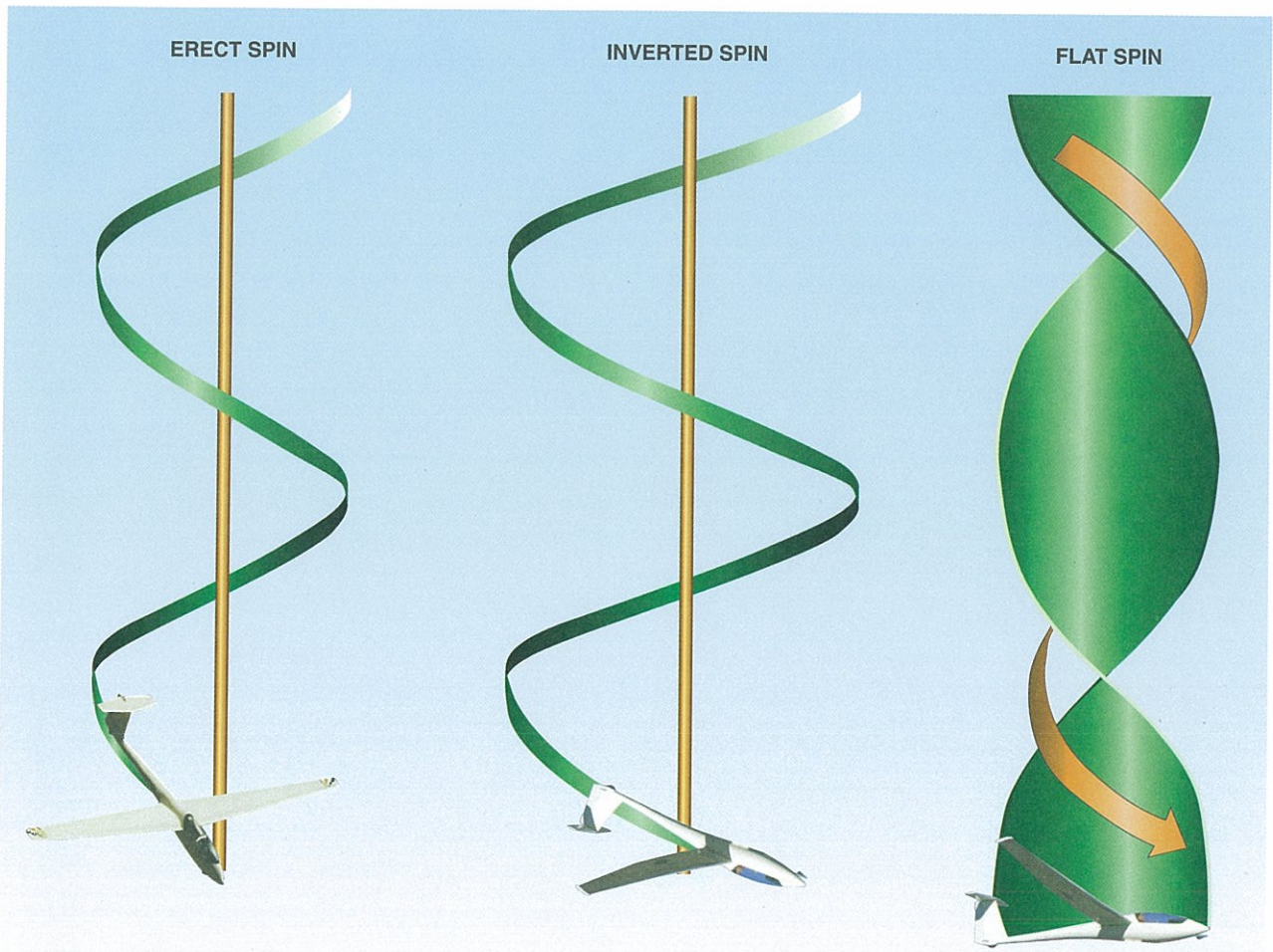
Figure 3-26. A spin can be upright or erect, inverted, or flat, depending on the roll and yaw motion of the glider.
