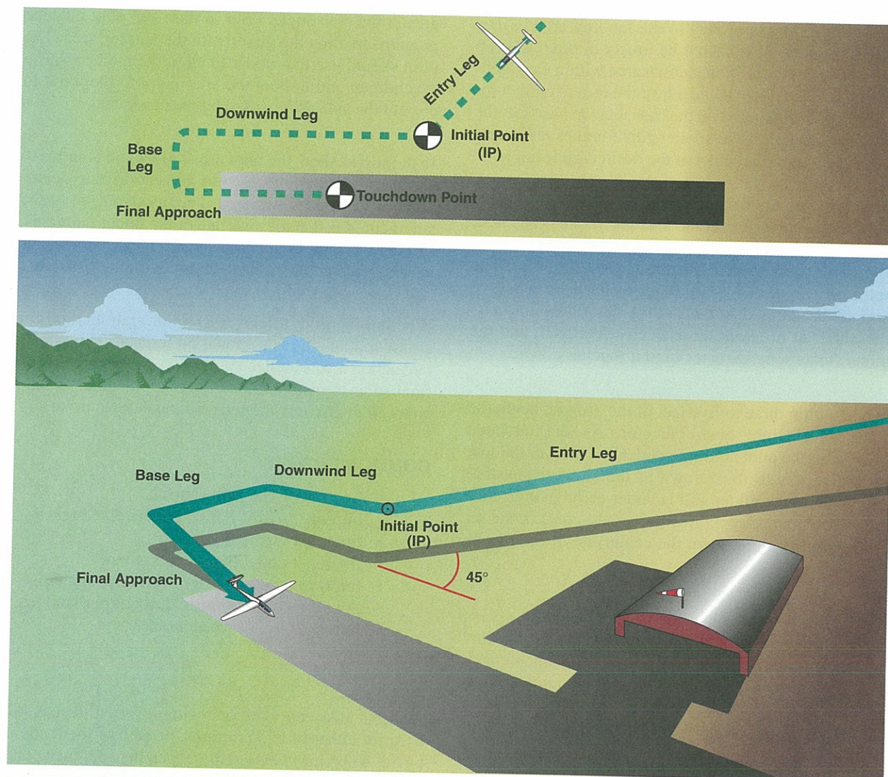
Figure 7-32. Traffic pattern.
