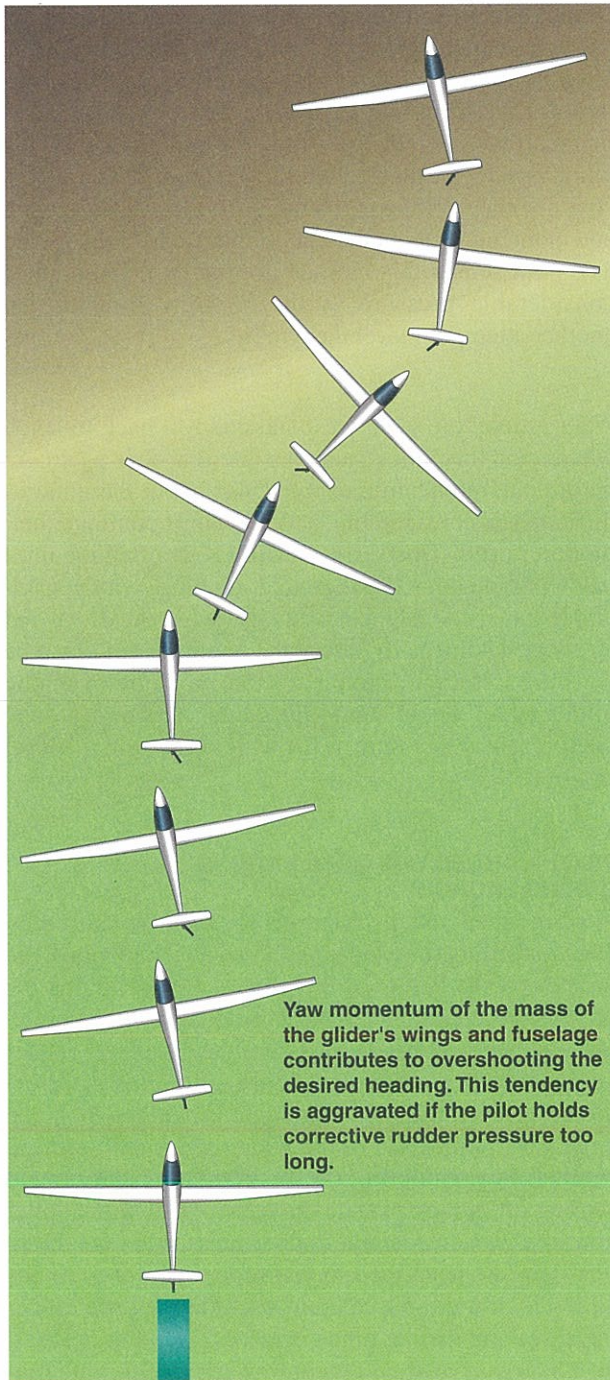
Figure 8-3. Pilot-induced yaw oscillations during takeoff roll.
