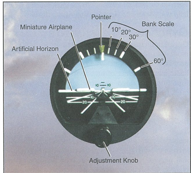
Figure 4-25. Attitude Indicator.
