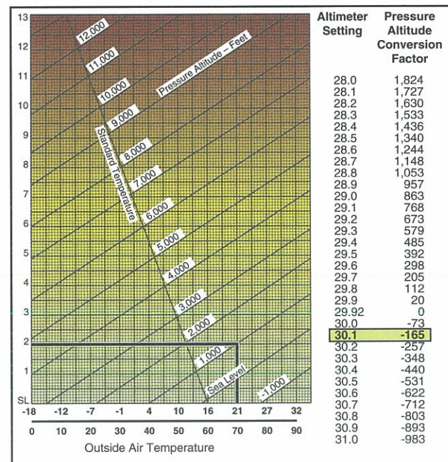
Figure 5-1. Density Altitude Chart.
