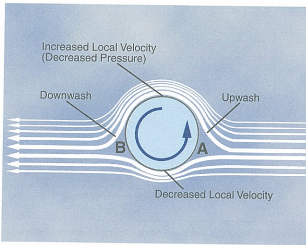
Figure 3-4. Magnus Effect.
