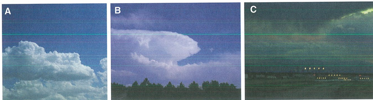
Figure 10-2. Photographs of (A) cumulus congestus, (B) cumulonimbus (Cb), (C) virga.
