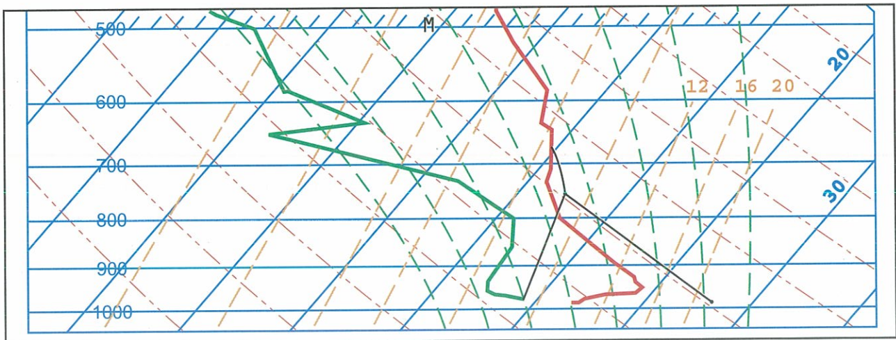
Figure 9-12. Skew-T from an actual sounding.
