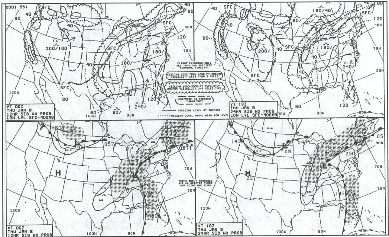
Figure 9-39. U.S. Low-Level Significant Weather Prognostic Chart.
