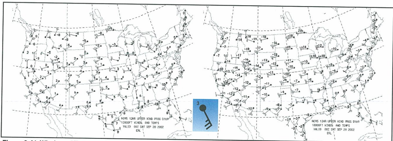
Figure 9-41. Winds and Temperatures Aloft (FD) chart.
