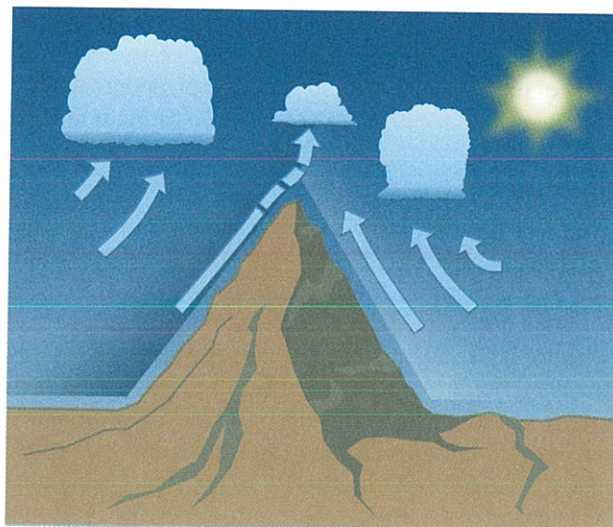
Figure 9-33. Mountain-top convergence.
