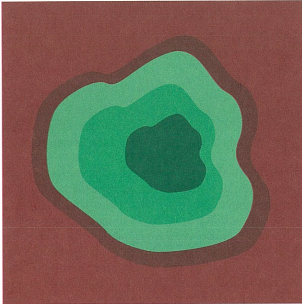
Figure 9-7. Cross-section through a thermal. Darker green is stronger lift, red is sink.
