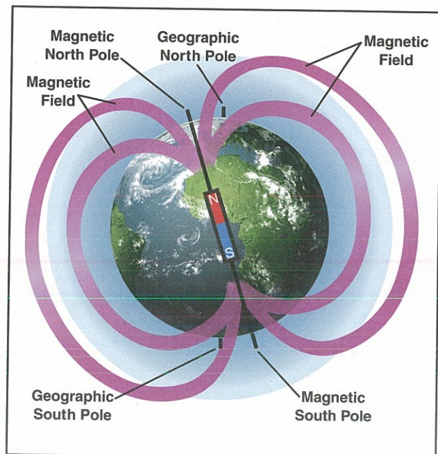
Figure 4-15. Earth magnetic force flow.
