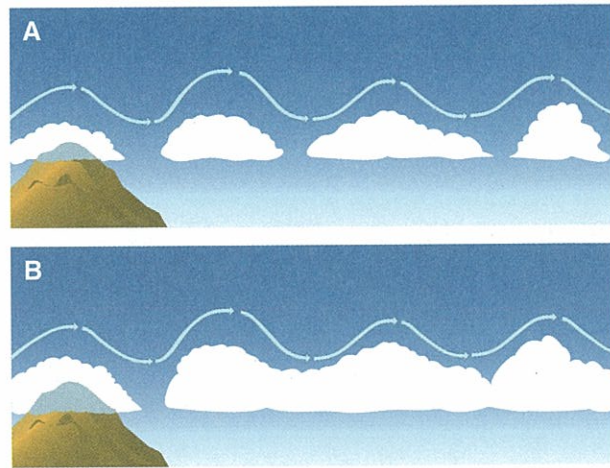
Figure 9-28. Small Föhn Gap under most conditions.
