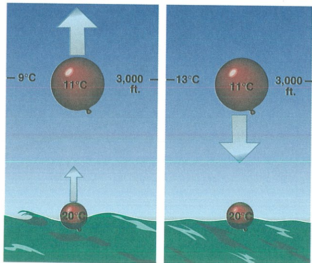
Figure 9-9. Stable and unstable parcels of air.
