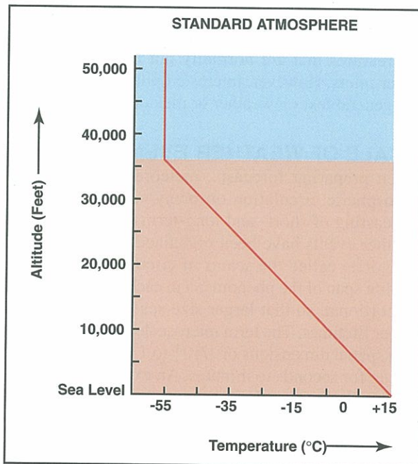
Figure 9-3. Standard Atmosphere.
