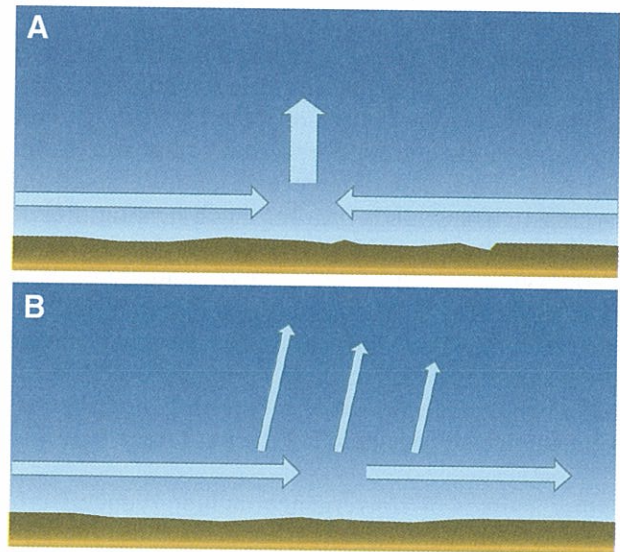
Figure 9-30. Convergence examples. (A) Wind from different directions. (B) Wind slows and “piles up.”
