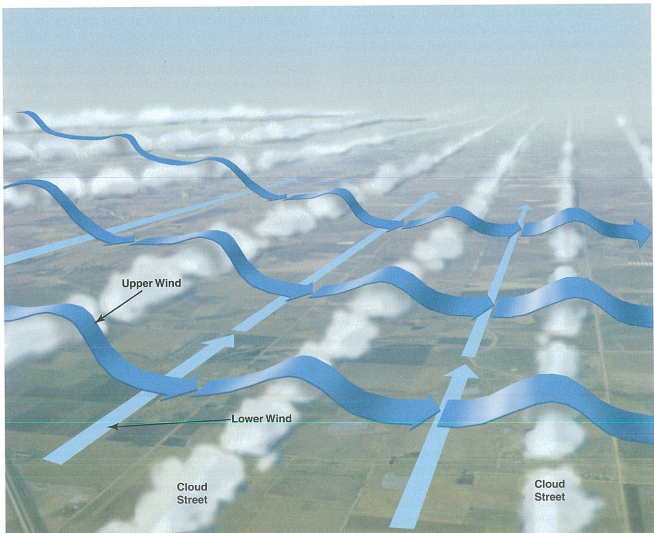
Figure 9-14. Cloud street wave.
