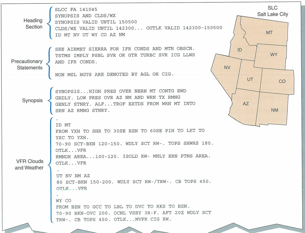
Figure 9-53. Aviation Area Forecast.
