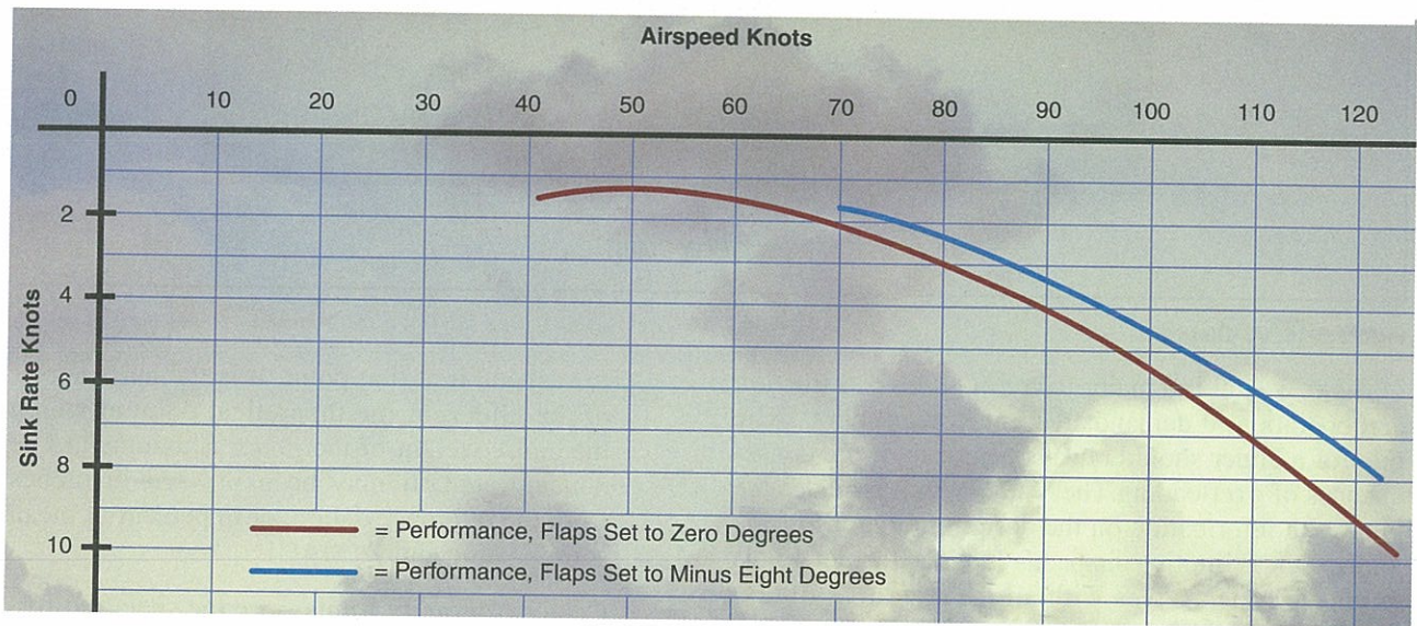
Figure 5-14. Performance polar with flaps at 0° and minus 8°.
