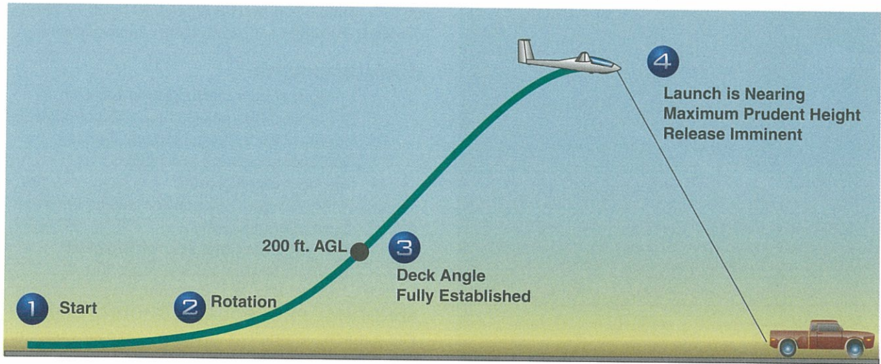
Figure 7-18. Ground launch takeoff profile.
