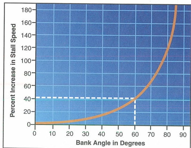
Figure 3-22. A glider's stall speed increases as the bank angle increases. For example, a 60° angle of bank causes a 40 percent increase in the glider's stall speed.
