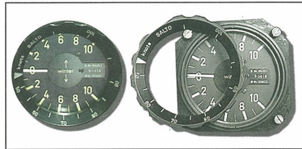
Figure 4-10. The MacCready ring.
