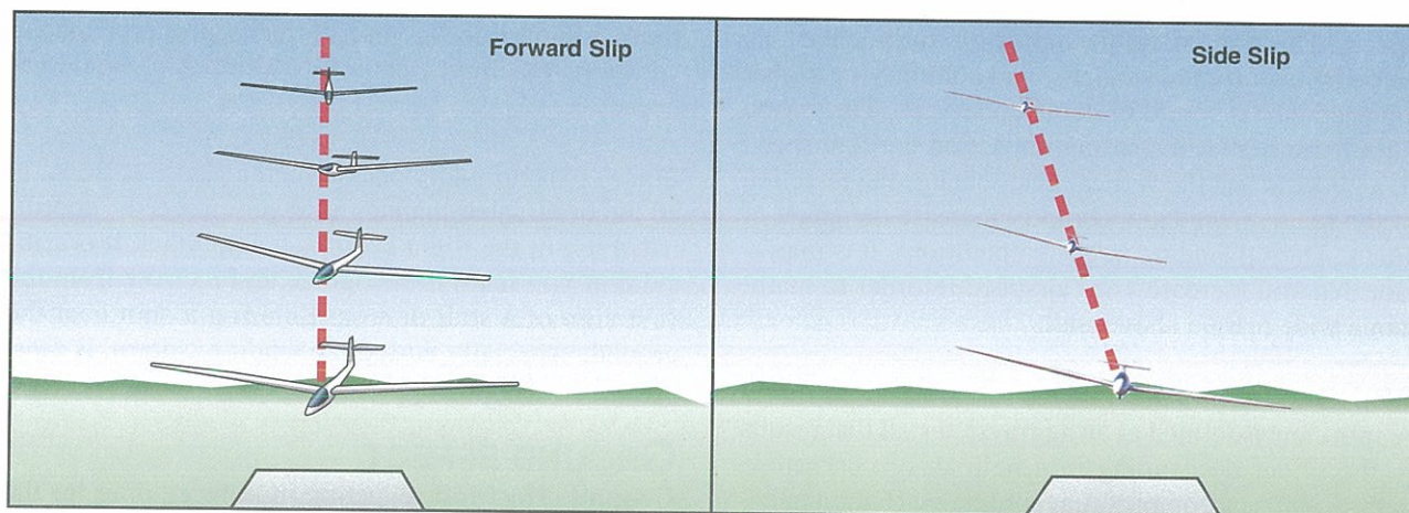
Figure 3-24. Two types of slips.
