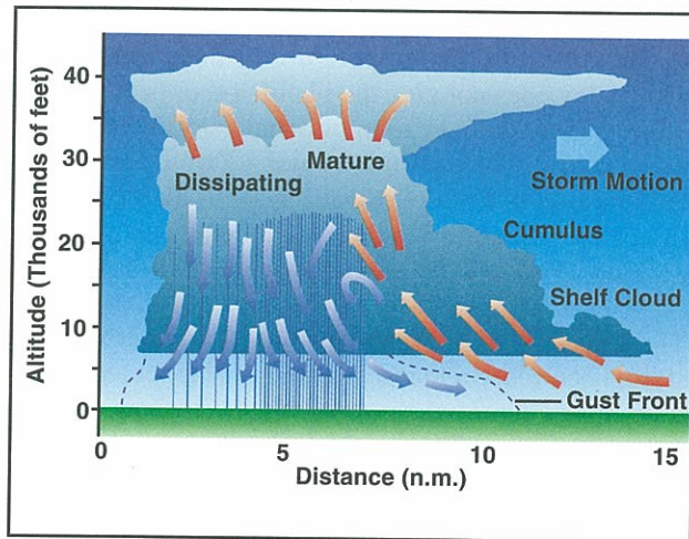
Figure 9-17. Multi-cell thunderstorm.
