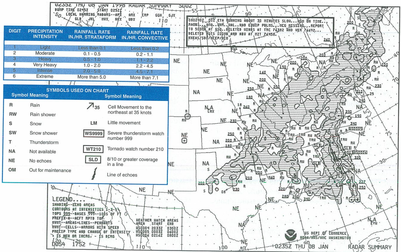
Figure 9-38. Radar Summary Chart.
