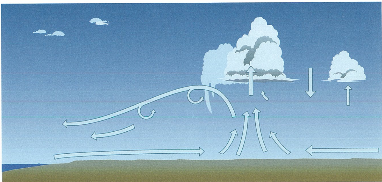
Figure 9-31. Sea-breeze front.
