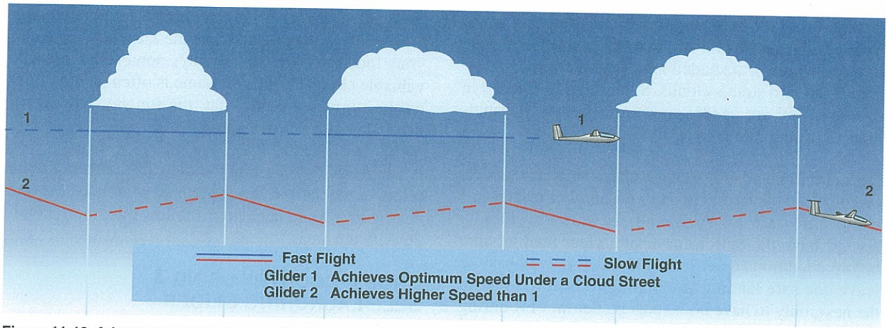
Figure 11-13. Advantage of proper speed to fly under a cloud street.
