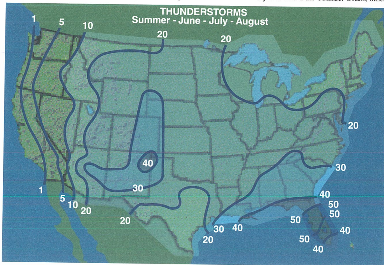
Figure 9-15. Thunderstorm frequency in the summertime.
