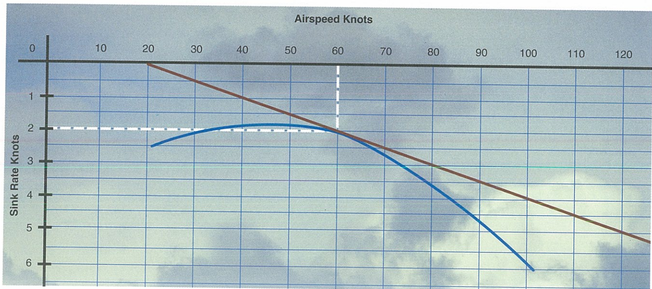
Figure 5-11. Best speed-to-fly in a 20-knot headwind.
