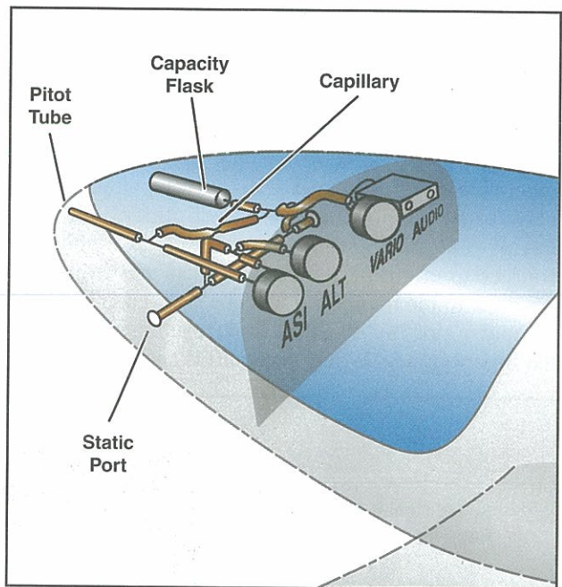
Figure 4-12. This is an example of a NETTO variometer system.
