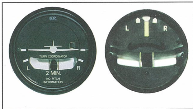
Figure 4-24. A turn coordinator and turn-and-slip indicator.
