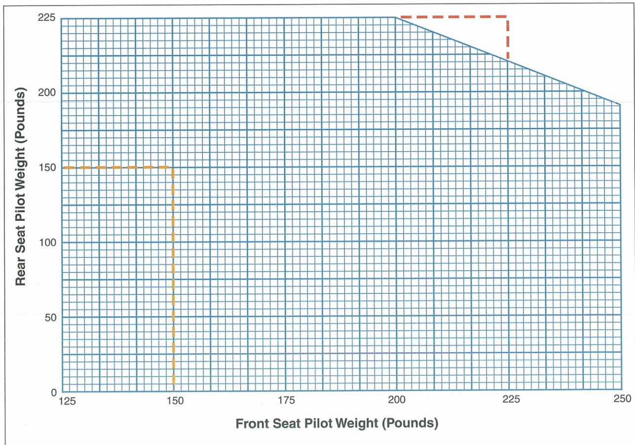
Figure 5-17. Graphic presentation of weight and balance envelope.
