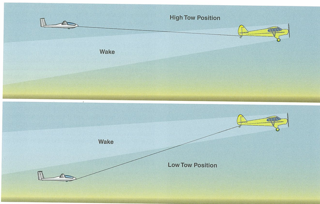
Figure 7-6. Aerotow climb-out.
