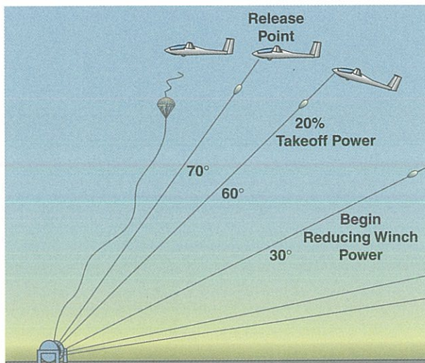
Figure 7-17. Wench procedures.
