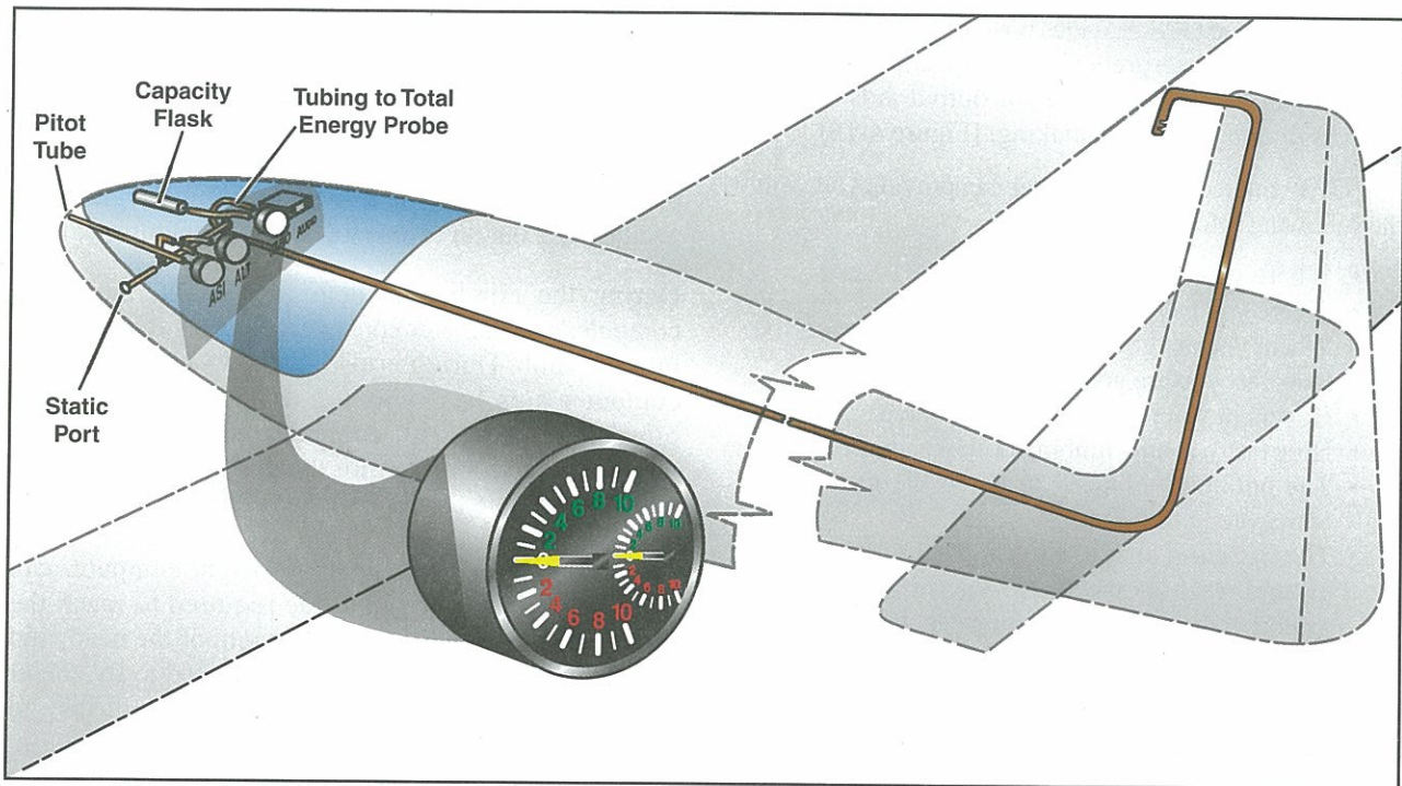
Figure 4-11. A total energy variometer system.
