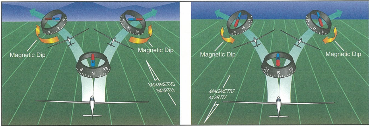
Figure 4-19. The left side of this figure shows the initial turning error that occurs during a turn from a northerly heading. The initial tendency of the magnetic compass in a turn from a southerly heading is shown on the right.
