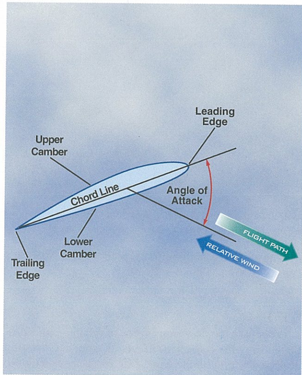
Figure 3-1. Aerodynamic terms of an airfoil.
