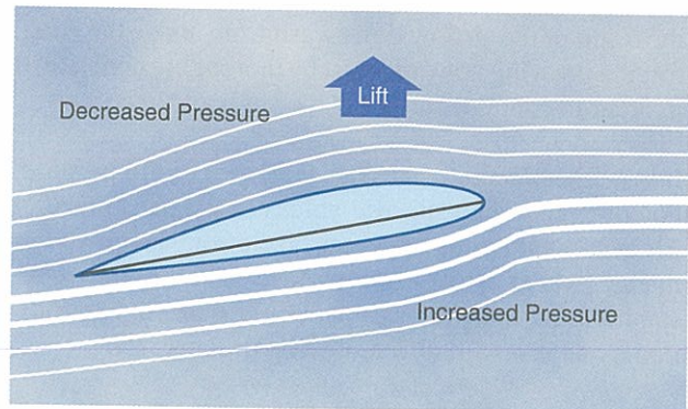
Figure 3-7. Lift is produced when there is decreased pressure above and increased pressure below an airfoil.
