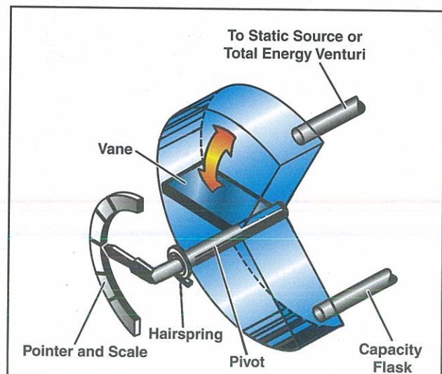
Figure 4-8. The mechanics of a variometer allow the instrument face to display small changes in pressure.
