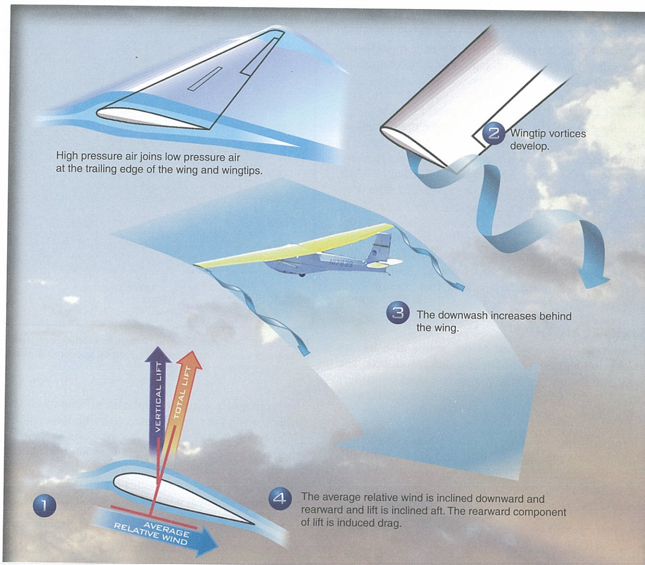
Figure 3-10. Induced drag is that part of total drag created by the production of lift. It occurs only when lift is being developed.
