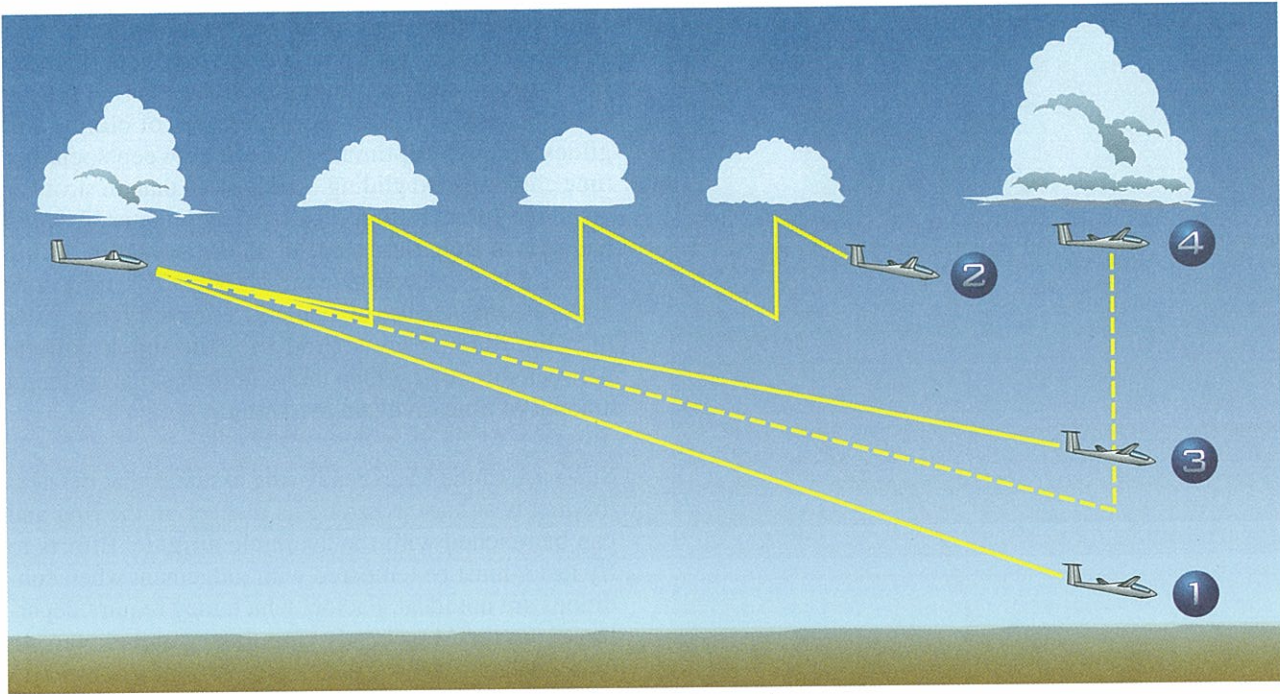
Figure 11-11. Examples of glides achieved for different MacCready ring settings.
