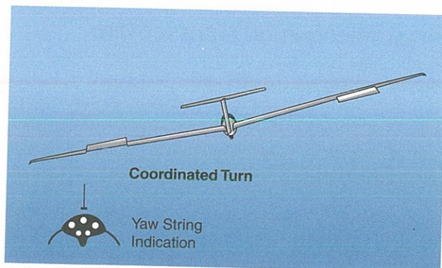
Figure 7-28. Coordinated turn.
