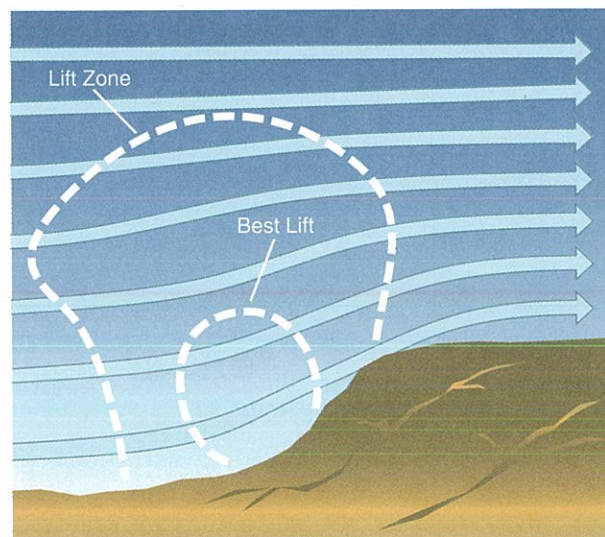
Figure 9-22. Slope soaring.
