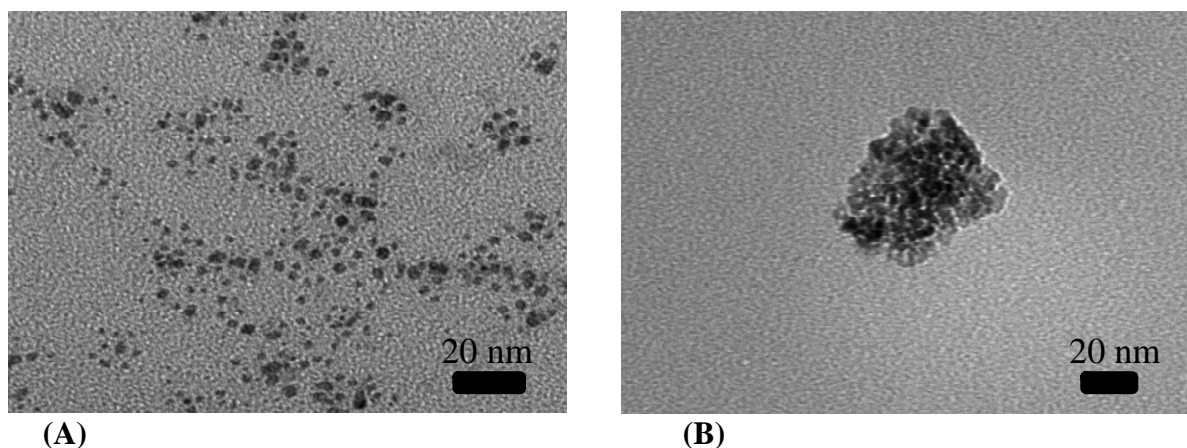
Figure 17. Transmission Electron Microscope (TEM) image of aerosol-generated TiO 2 nanoparticles.
