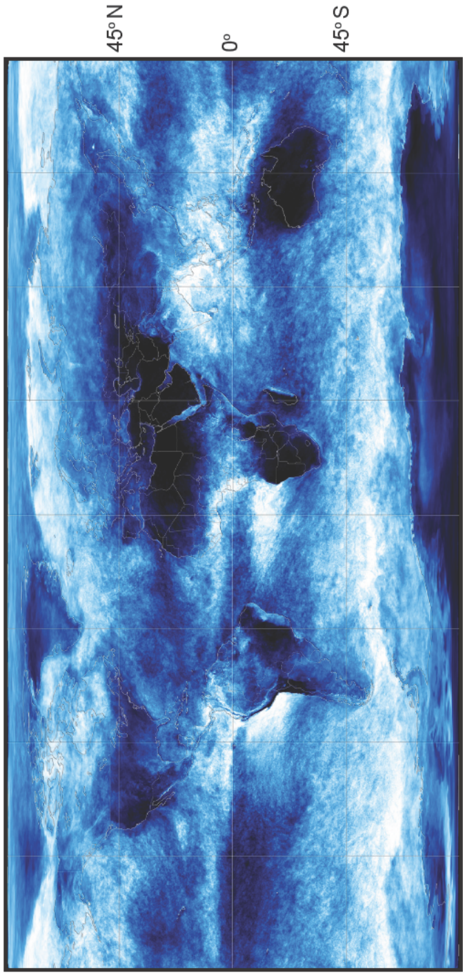
Cloud Fraction: September 2007
