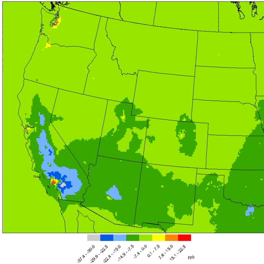
FIGURE 4-11. DIFFERENCE IN SIMULATED DAILY MAXIMUM 8-HOUR OZONE CONCENTRATION (PPB) FOR THE WUS DOMAIN FOR 15 AUGUST: 2020 WITH-CAAA MINUS 2020 WITHOUT-CAAA SCENARIOS
