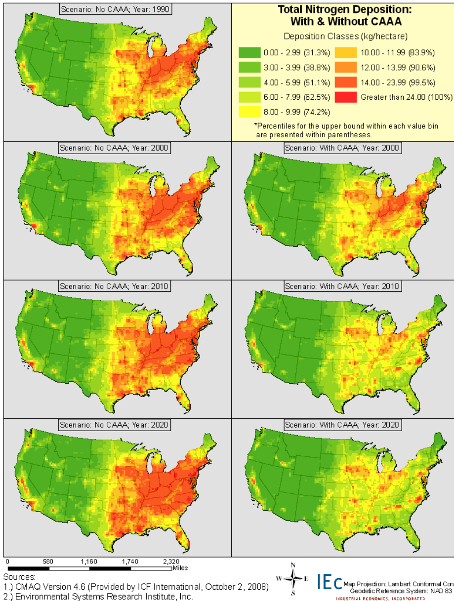
FIGURE 6-3. TOTAL NITROGEN DEPOSITION ESTIMATES FOR 1990, 2000, 2010, AND 2020 WITH AND WITHOUT THE CAAA 64, 65
