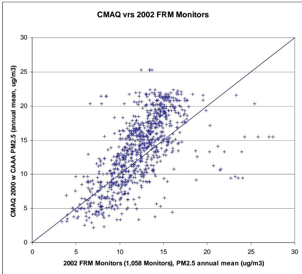
FIGURE 4-3. SCATTER PLOT OF DIRECT CMAQ ESTIMATES AND 2002 PM 2.5 MONITORS
