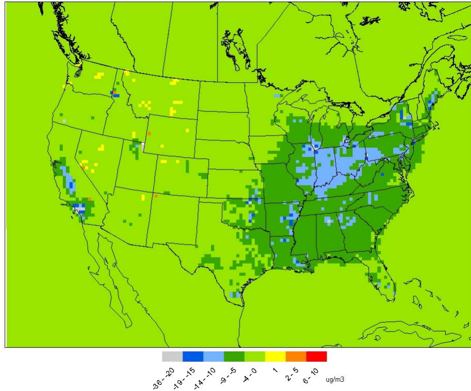
FIGURE 4-7. DIFFERENCE IN CMAQ SIMULATED MATS ADJUSTED ANNUAL AVERAGE PM2.5 SPECIES CONCENTRATION ( \mu\text{GM}^{-3} ) FOR THE CONUS DOMAIN: 2020 WITH-CAAA MINUS 2020 WITHOUT CAAA SCENARIOS
