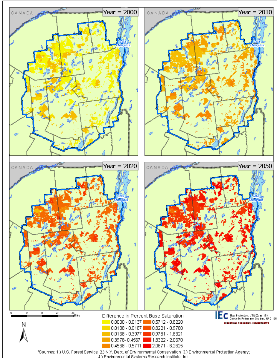
FIGURE 6-11. DIFFERENCES IN PERCENT BASE SATURATION VALUES WITH AND WITHOUT THE CAAA IN FORESTED RESOURCE MANAGEMENT AREAS IN ADIRONDACK PARK 80, 81
