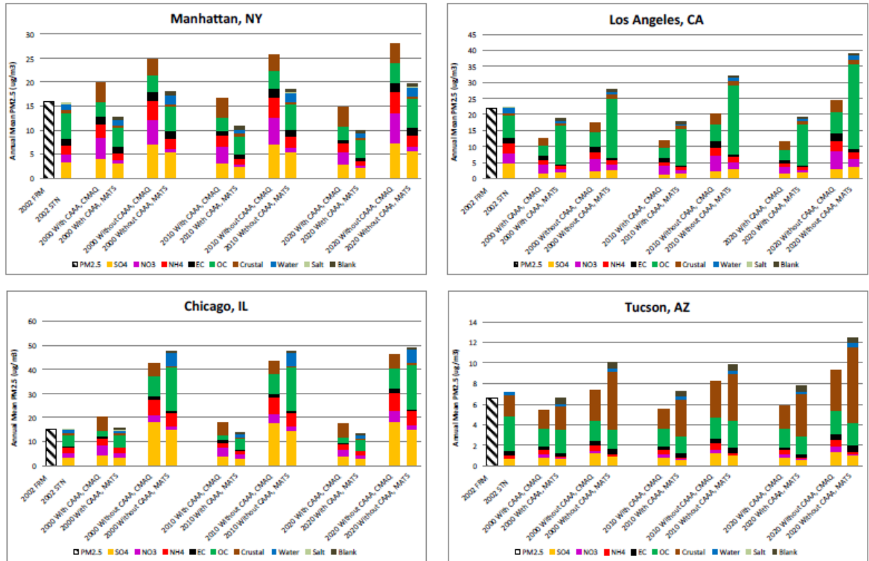
FIGURE 4-5. COMPARISON OF CMAQ, MATS, AND MONITOR DATA FOR FOUR SELECTED CITIES
