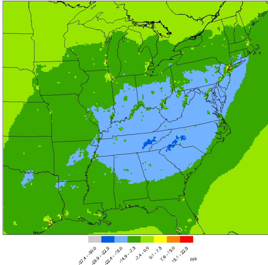
FIGURE 4-9. DIFFERENCE IN SIMULATED DAILY MAXIMUM 8-HOUR OZONE CONCENTRATION (PPB) FOR THE EUS DOMAIN FOR 15 JULY: 2020 WITH-CAAA MINUS 2020 WITHOUT-CAAA SCENARIOS
