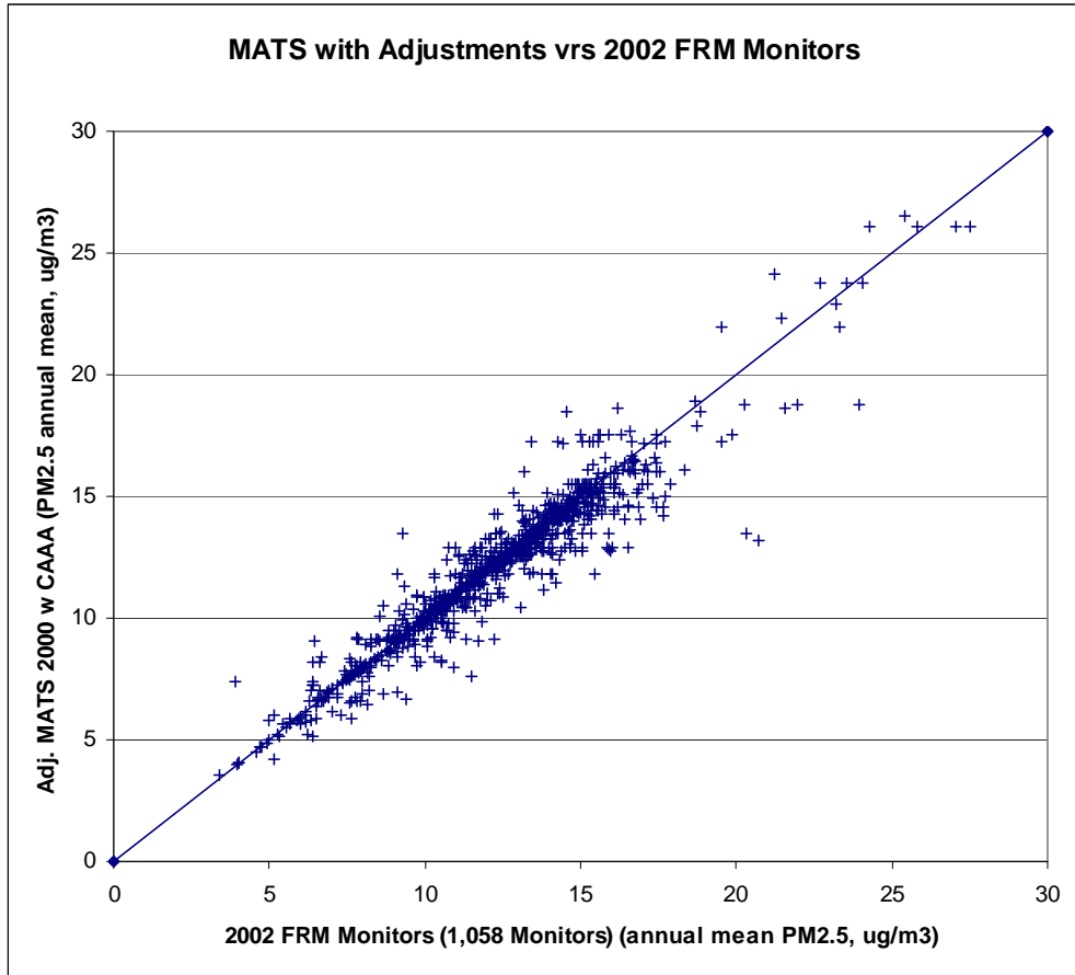
FIGURE 4-4 SCATTER PLOT OF MATS ESTIMATES AND 2002 PM 2.5 MONITORS
