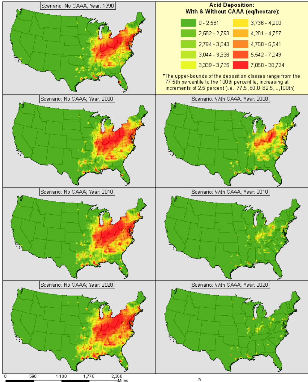
FIGURE 6-2. COMBINED NO x AND SO x DEPOSITION ESTIMATES FOR 1990, 2000, 2010, AND 2020 WITH AND WITHOUT THE CAAA
