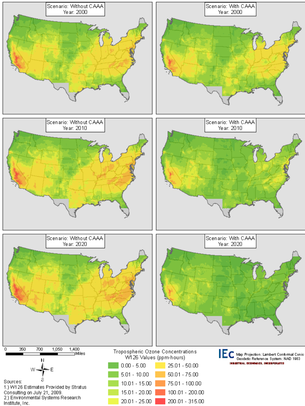
FIGURE 6-4. W126 CUMULATIVE TROPOSPHERIC OZONE SEASON MEASURES FOR 2000, 2010, AND 2020 WITH AND WITHOUT THE CAAA
