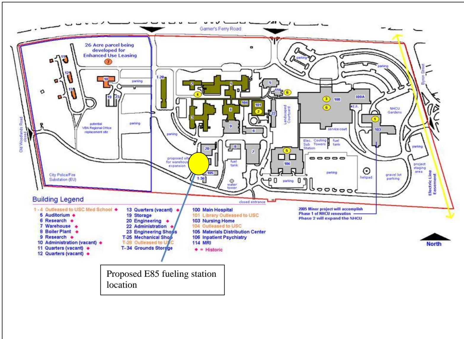
Figure 2-3. Facility map highlighting the preferred site for the E85 fueling station at the Dorn VAMC adjacent to Building T25
