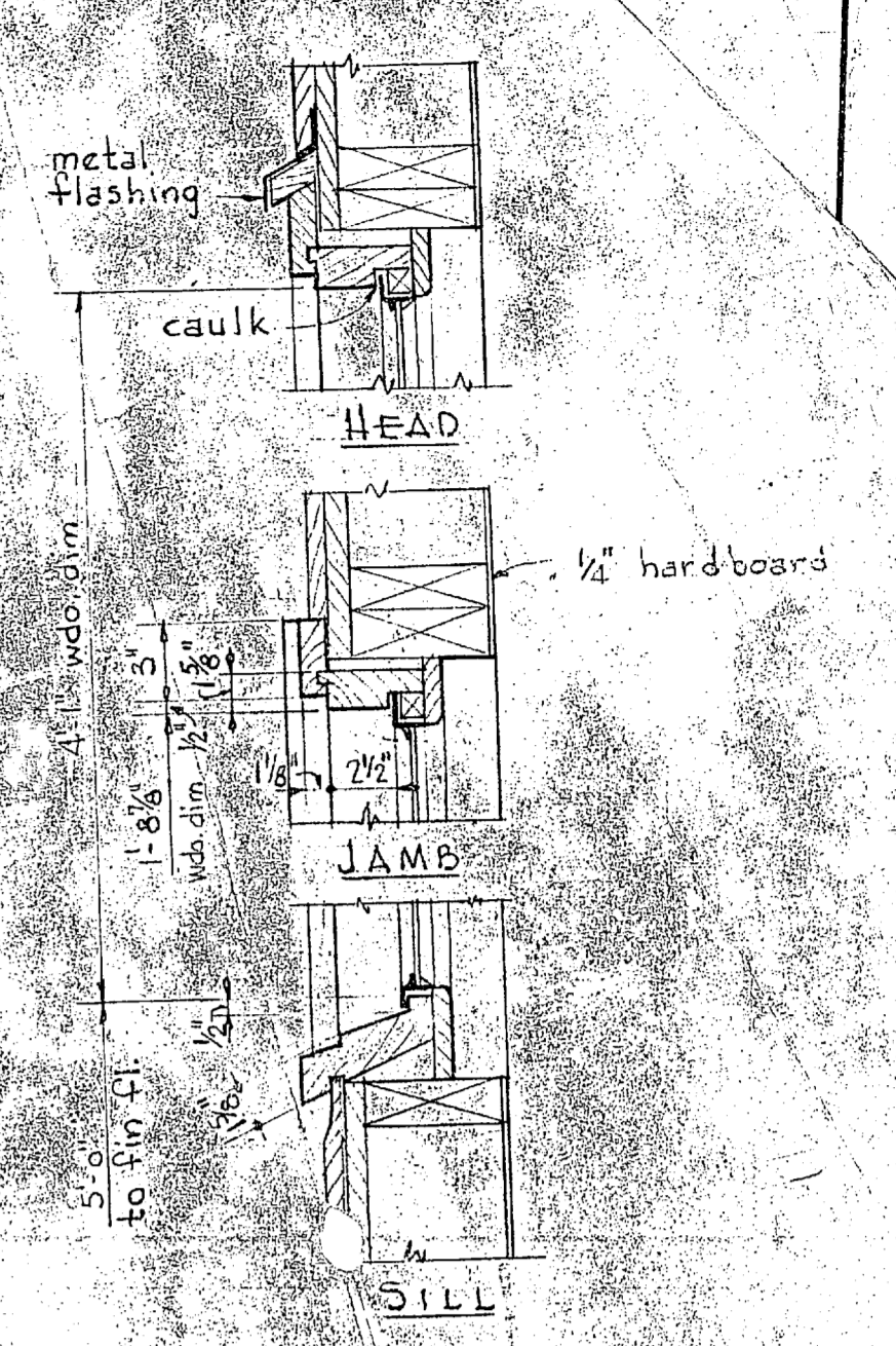
WINDOW DETAIL Scale: 1/2" = 1'-0"
