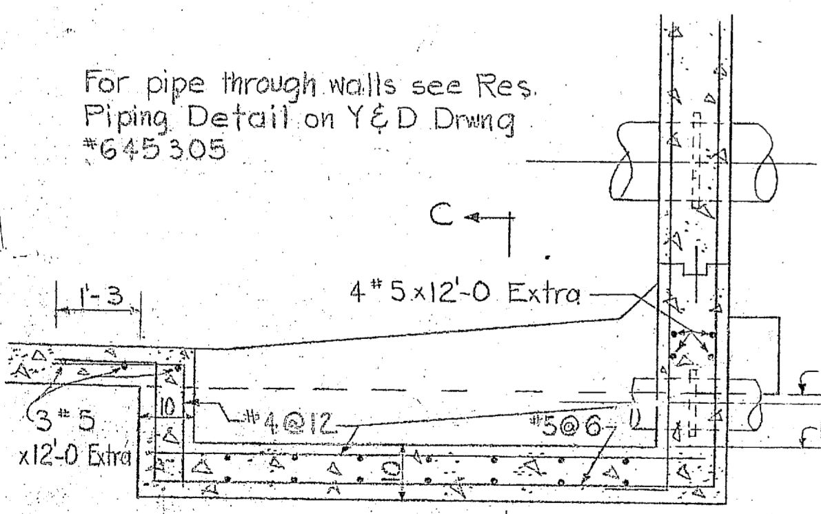
SECT. B-B
