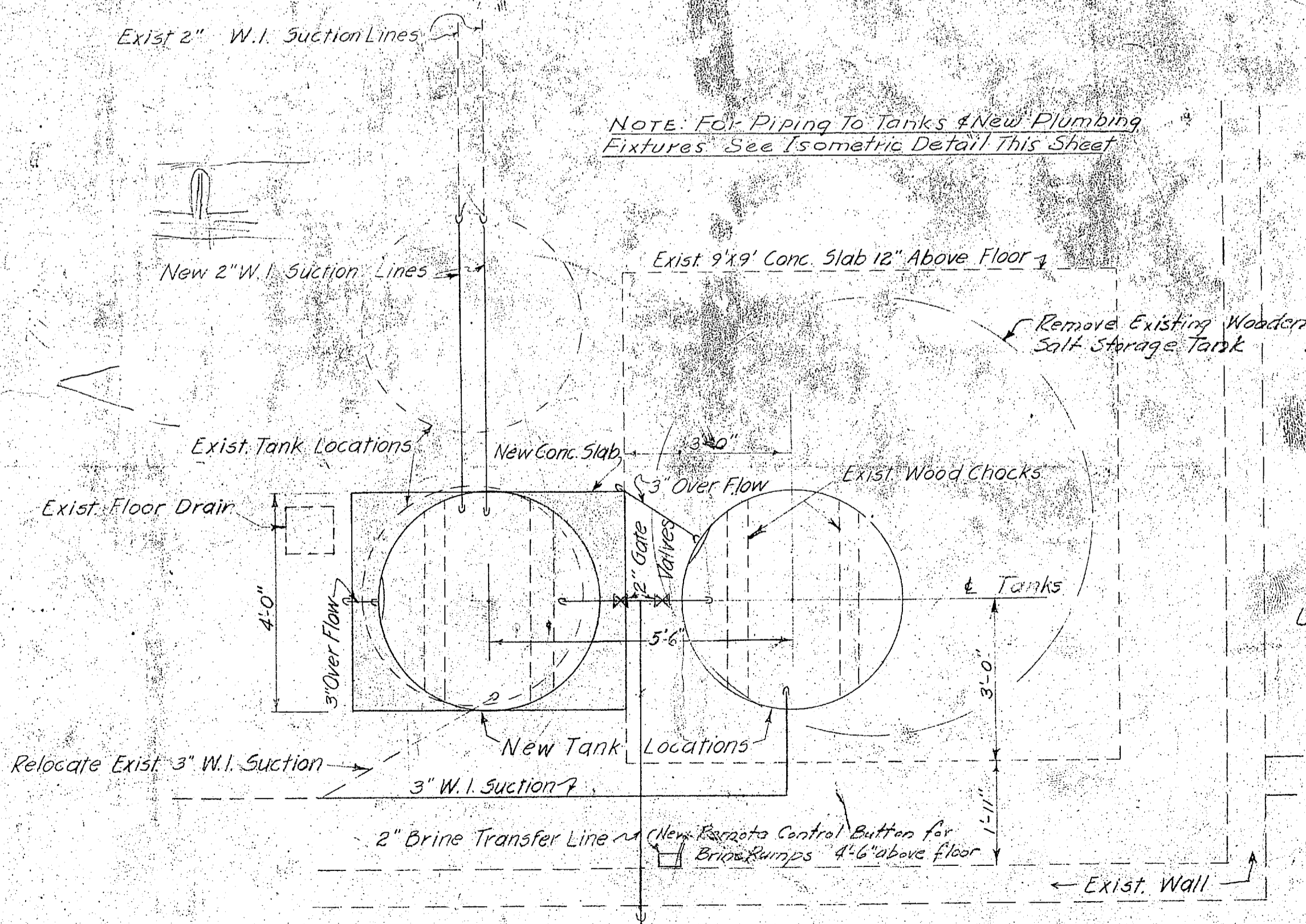
PLAN NEW LOCATIONS OF EXISTING BRINE MEASURING TANKS SCALE 3/4"=1'-0"
