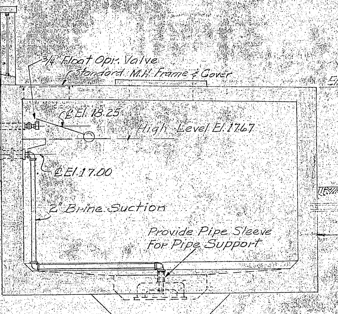
SECTION E-E SCALE 3/8" = 1'-0"
