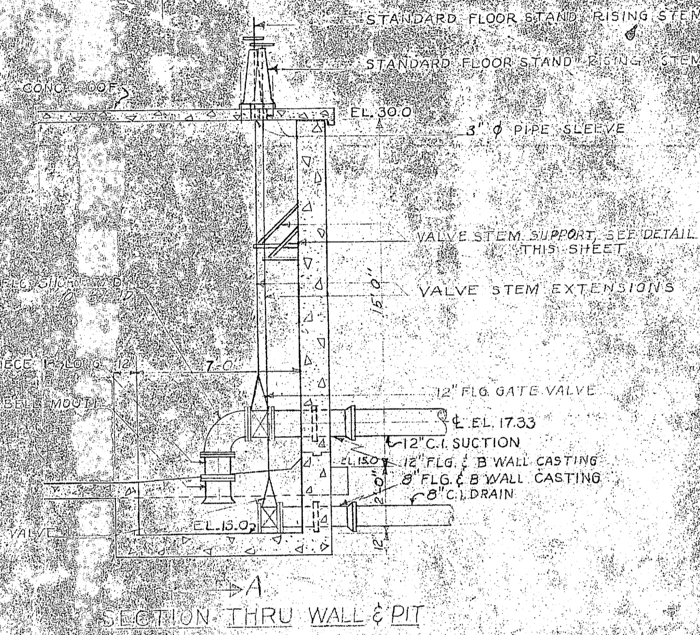
RESERVOIR PIPING DETAIL OF SUCTION AND DRAIN LINES NOTE: INFLUENT LINE THROUGH WALL TO BE AT SAME ELEVATION AS SUCTION LINE. USE RISING STEM FLOOR STAND FOR LOCATIONS SEE Y & D DWG. NO. 645306
