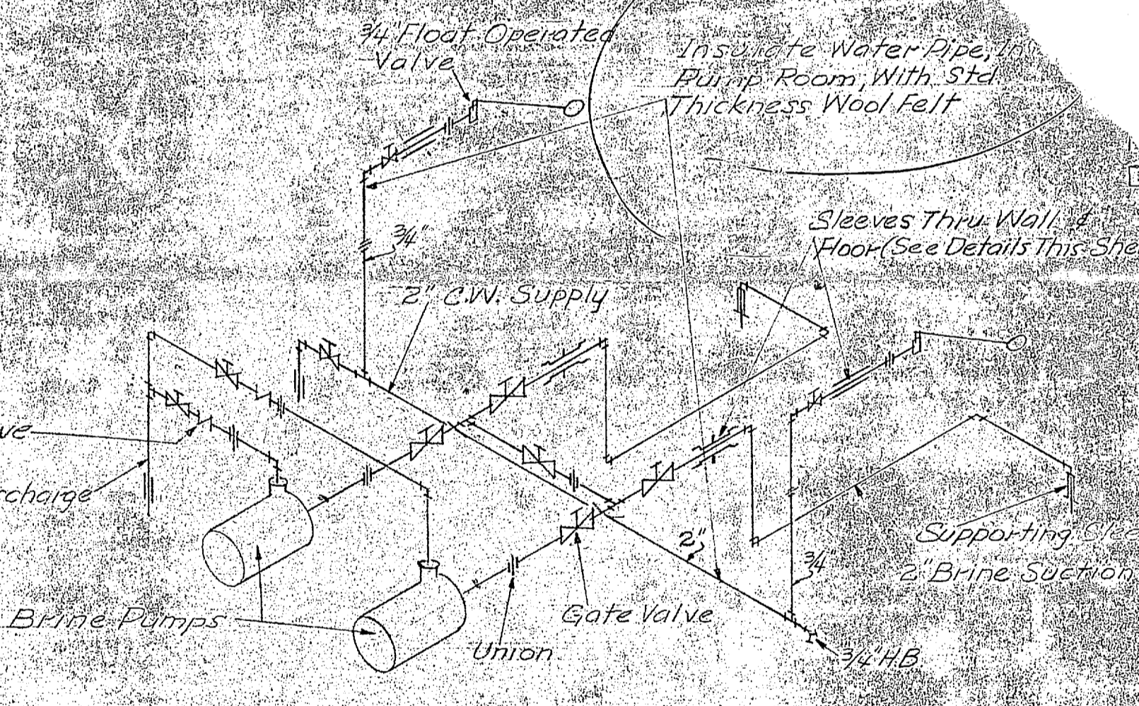
ISOMETRIC WATER & BRINE PIPING AT SALT STORAGE TANKS No Scale
