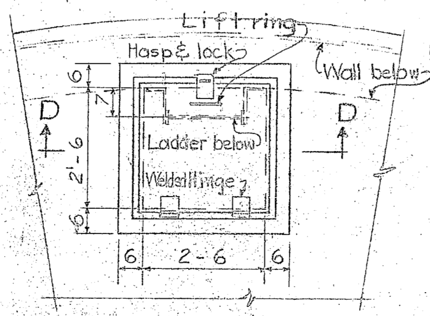
ACCESS M.H. DETAILS (2 REQUIRED) Scale 1/2" = 1'-0"
