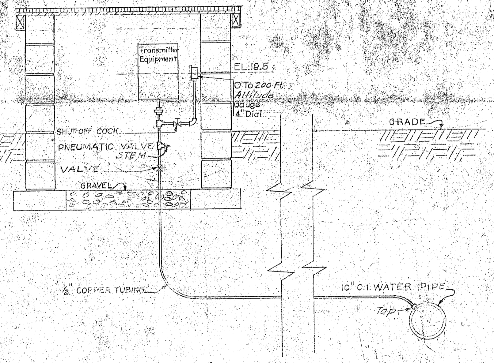
DETAIL OF PIPING TO TRANSMITTER SCALE 3/4"=1'
