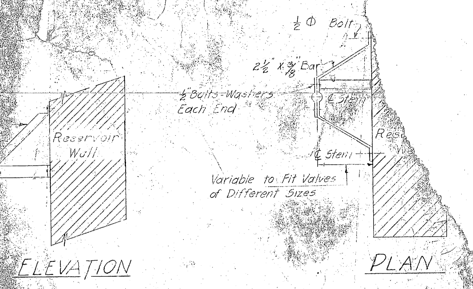
DETAIL OF VALVE STEM SUPPORT SCALE 1"=1'-0"
