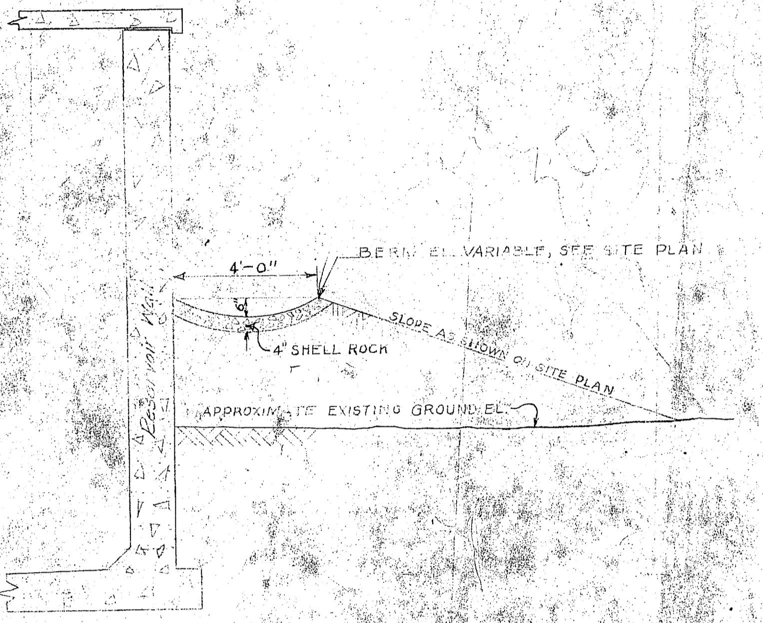
DETAIL OF SHELL ROCK GUTTER ON RESERVOIR BERM
