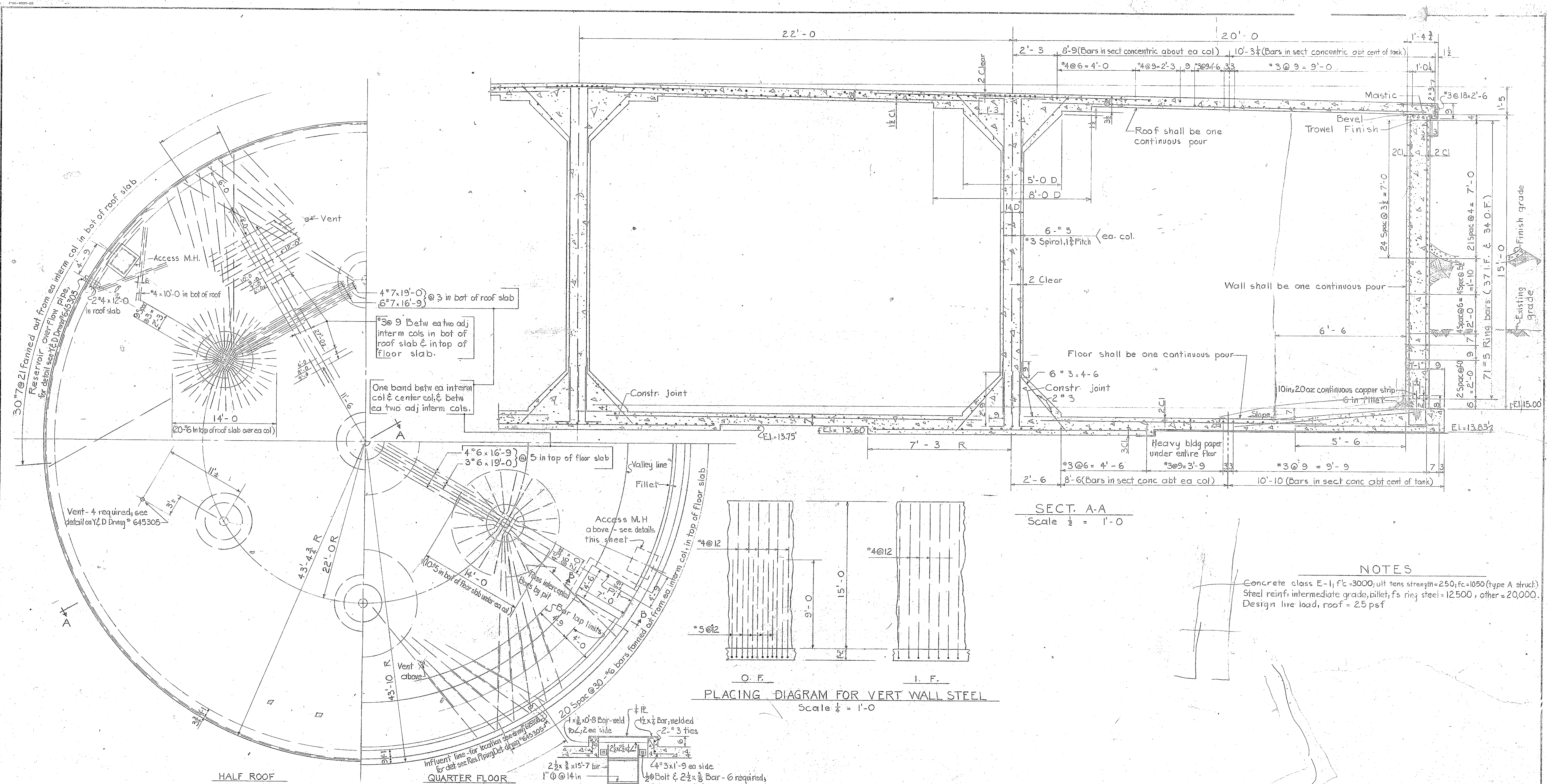
PLAN Scale 1/8" = 1'-0"
