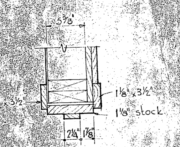
EXTERIOR DOOR JAMB Scale: 1/2" = 1'-0"
