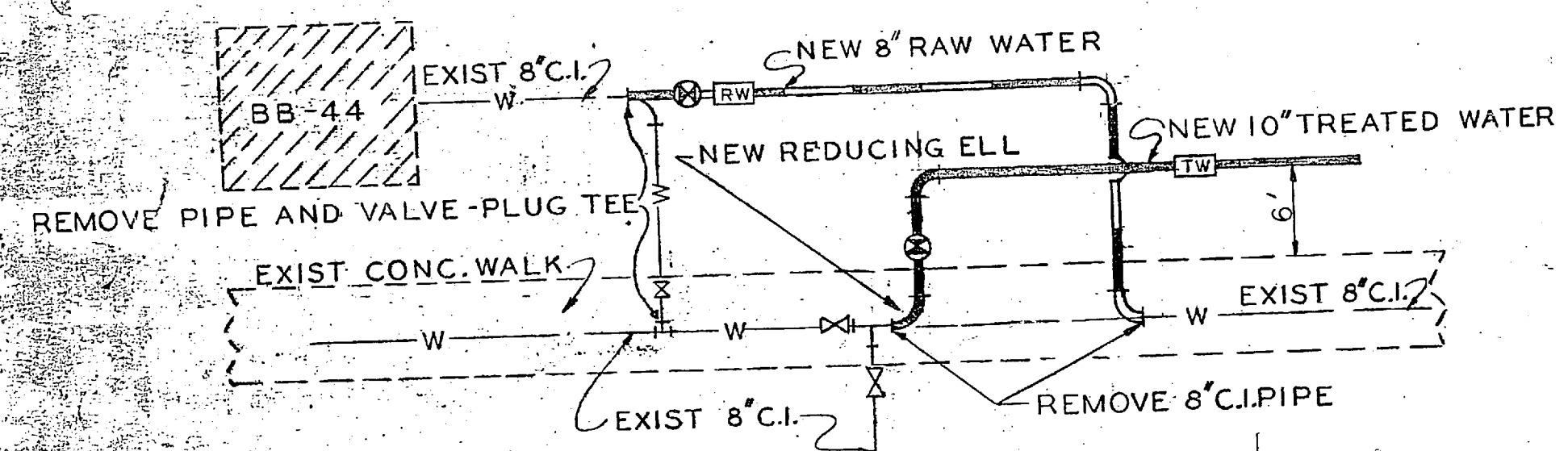
ENLARGEMENT SHOWING TIE-INS FOR RAW AND TREATED WATER MAINS SCALE 1"=10'
