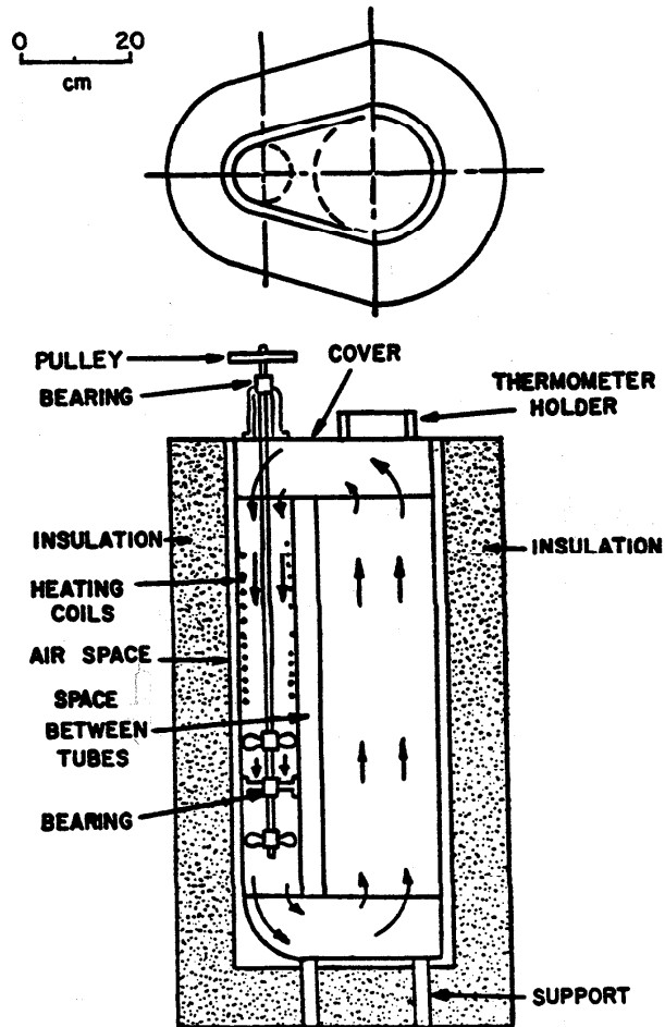
Figure 3.5. Oil bath and water bath.
