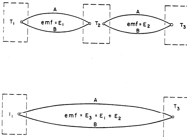
Figure 2.8. Emfs are additive for temperature intervals.
