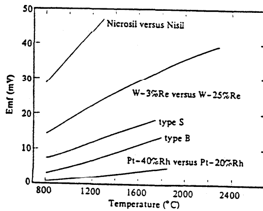
Figure 2.4. Temperature-emf relationships of some high-temperature thermocouples
