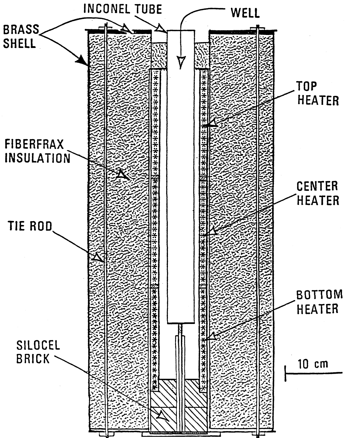
Figure 3.11. Freezing point furnace for gold and silver.
