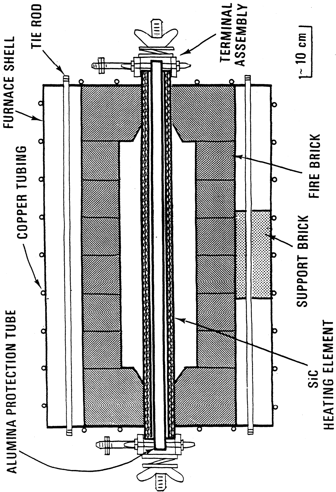
Figure 3.3. Silicon carbide tube furnace (50 to 1600 °C).
