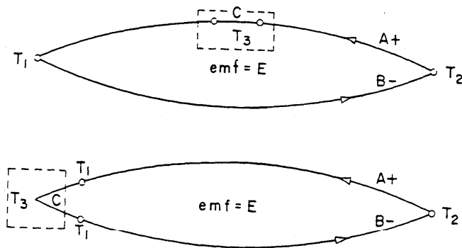
Figure 2.6. Emf(E) unaffected by third material, C.
