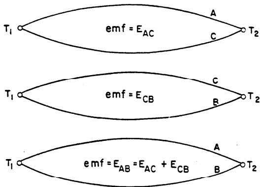
Figure 2.7. Emfs are additive for materials.
