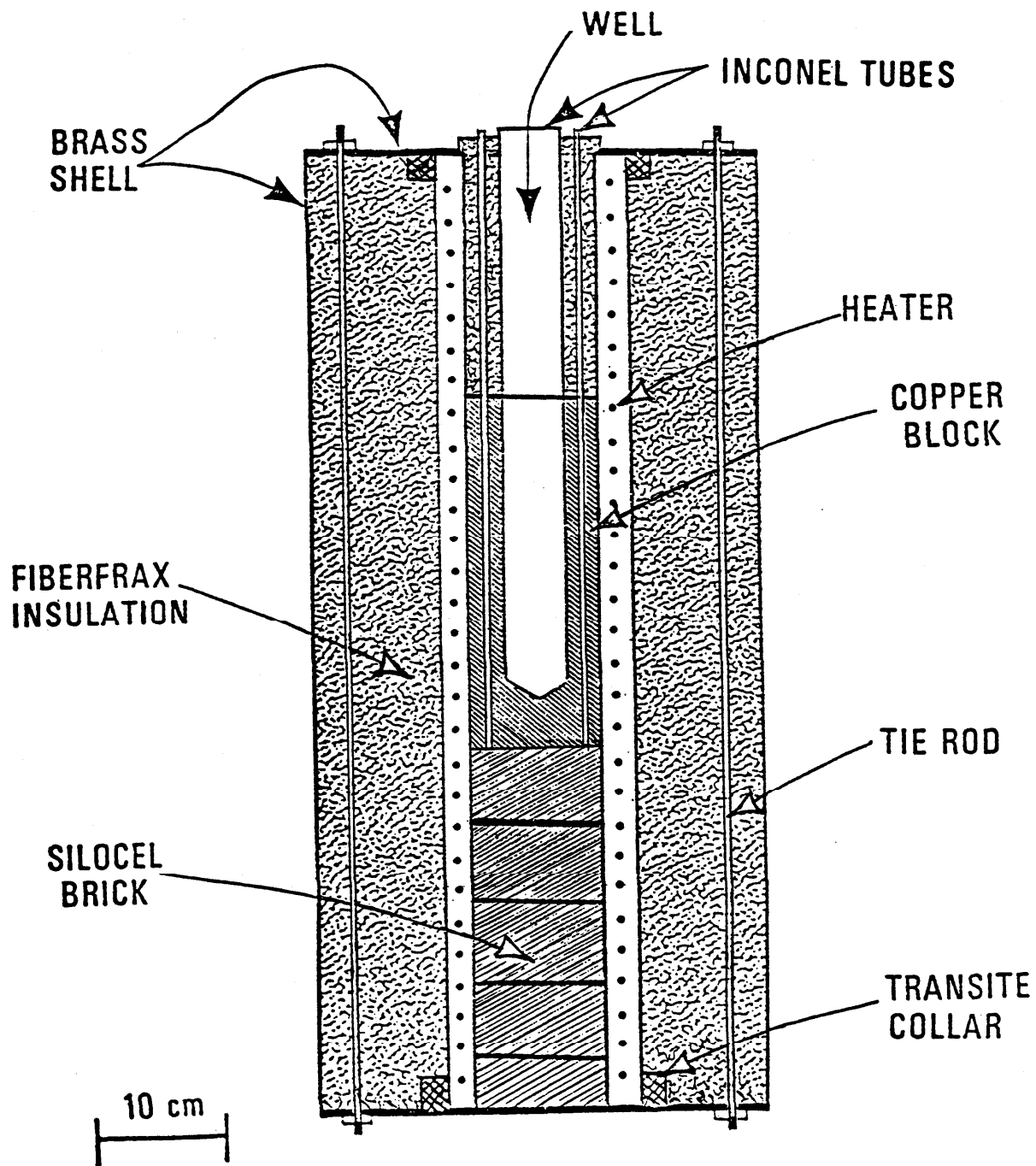
Figure 3.12. Freezing point furnace for antimony and zinc.
