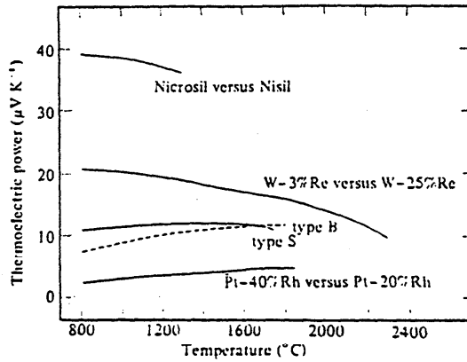
Figure 2.5. Thermoelectric power of some high-temperature thermocouples.
