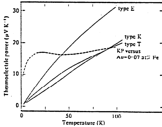
Figure 2.2. Thermoelectric power of some low-temperature Thermocouples.
