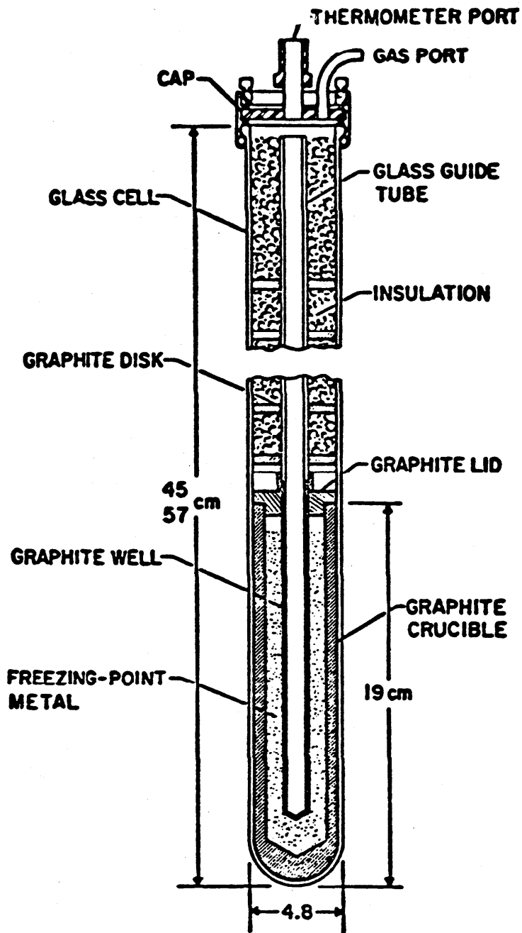
Figure 3.10. Metal freezing-point cell.
