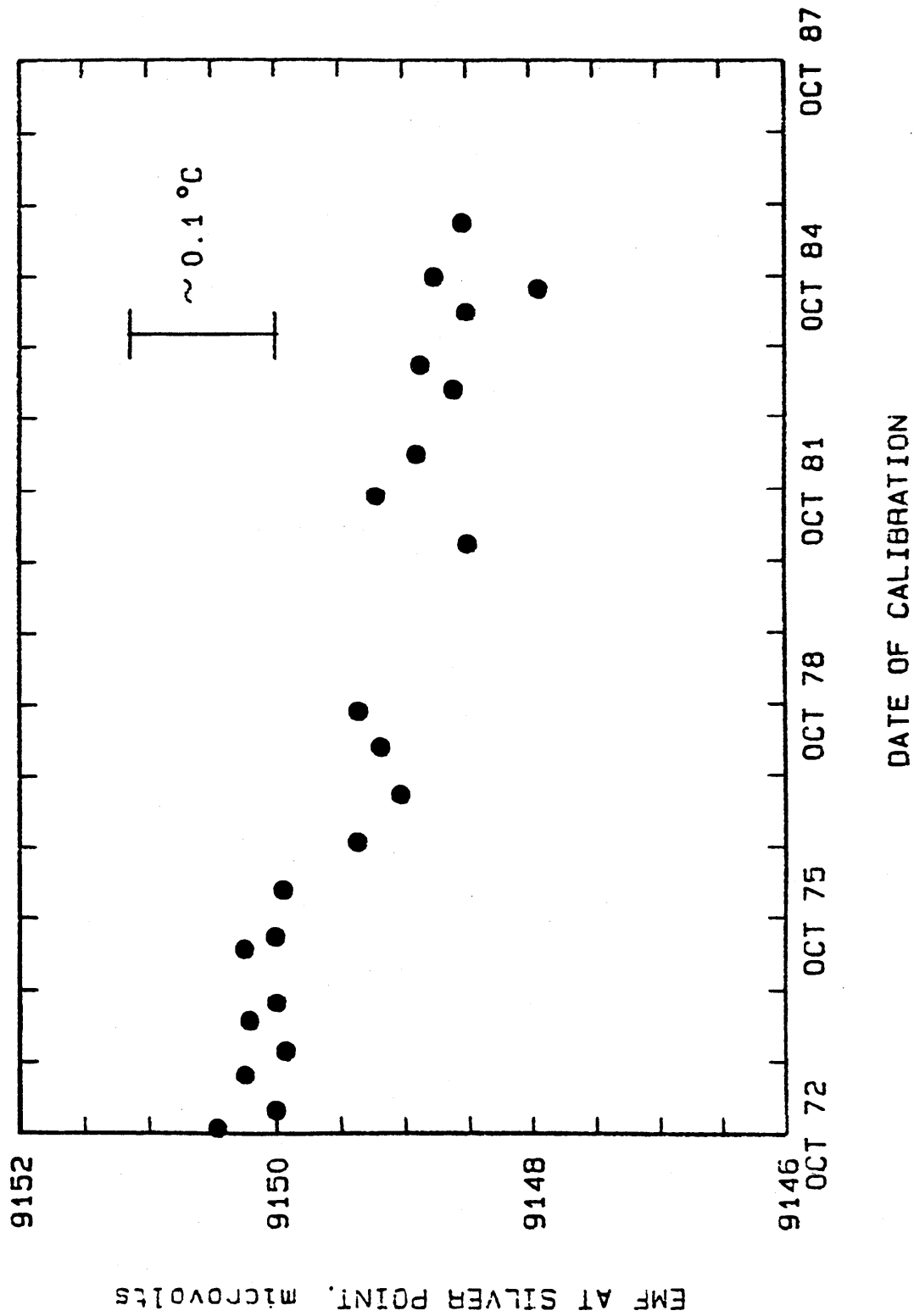
Figure 4.24. Calibration history of type S standard thermocouple SC-72-2 at the silver point (961.93 °C).
