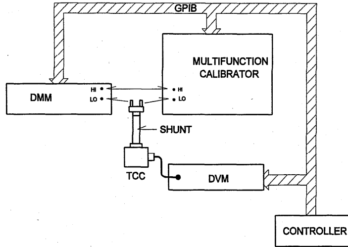
Fig. 10. Setup for characterizing ACI function of MCS calibrator using a TCC.
