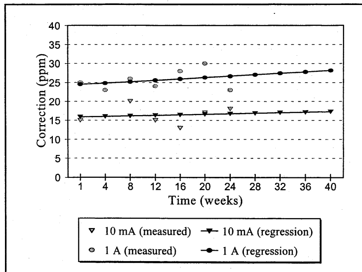
Fig. 5. Control chart with measured and predicted corrections for the MCS calibrator for DCI.
