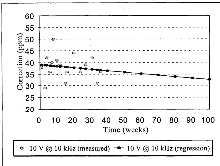
Fig. 9. Control chart with measured and predicted corrections for the MCS calibrator at 10 V and 10 kHz.
