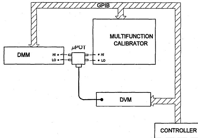
Fig. 8. Setup for characterizing the ACV function of the MCS using a \mu pot.
