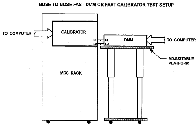
Fig. 12. Setup to calibrate a test DMM using the characterized MCS calibrator.
