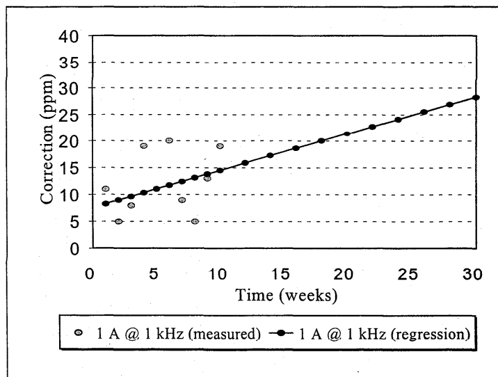
Fig. 11. Control chart with measured and predicted corrections for the MCS calibrator for ACI.
