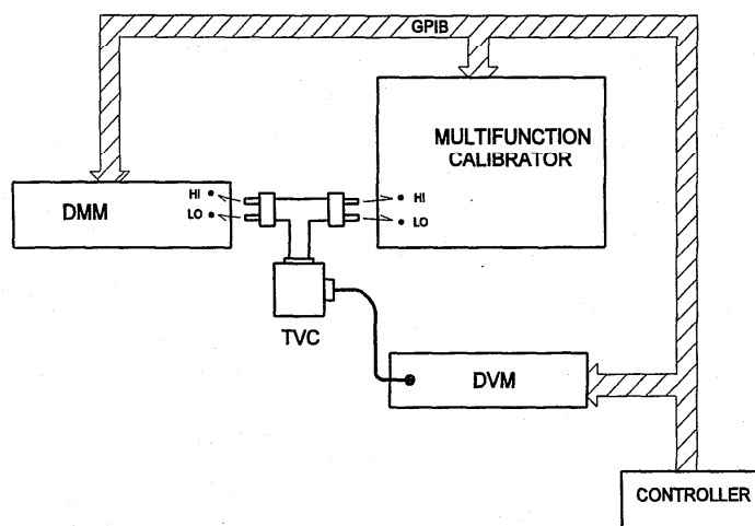
Fig. 7. Setup for characterizing the ACV function of the MCS using a multirange TVC.
