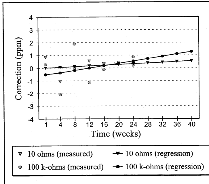
Fig. 6. Control chart with measured and predicted corrections for the MCS calibrator for DCR.
