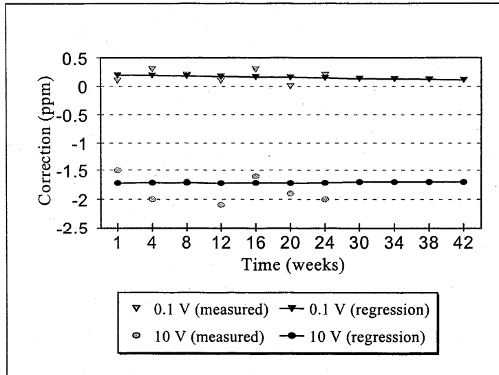
Fig. 4. Control chart with measured and predicted corrections for the MCS calibrator for DCV.
