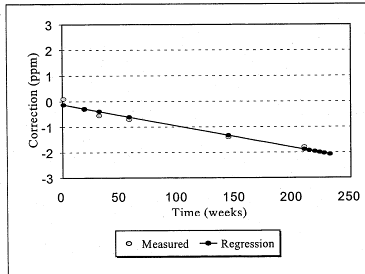
Fig. 3. Control chart with measured and predicted corrections for the zener reference.
