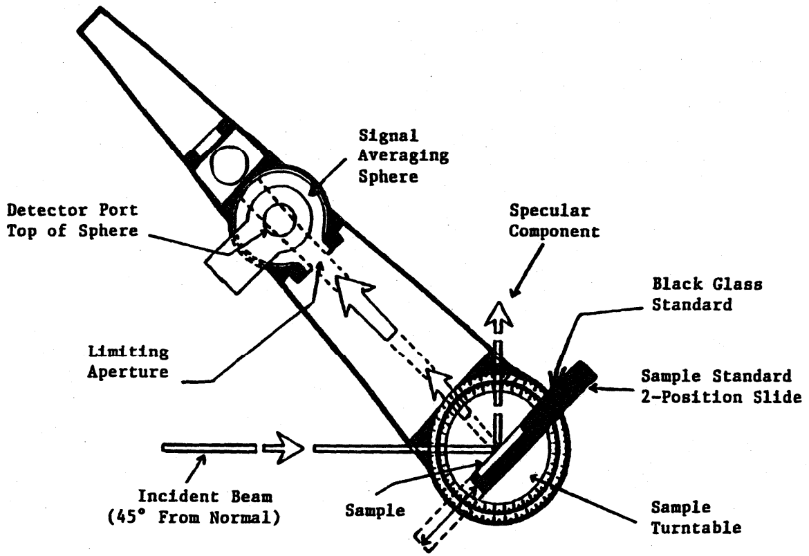
Figure 2. 45°/0° Reflectometer System (Top View)
