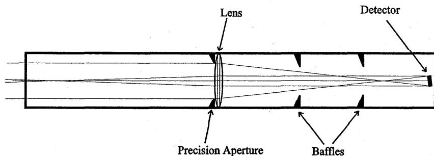
Figure 3.4. Cross-section of the detection system on the goniometer system of the STARR instrument.
