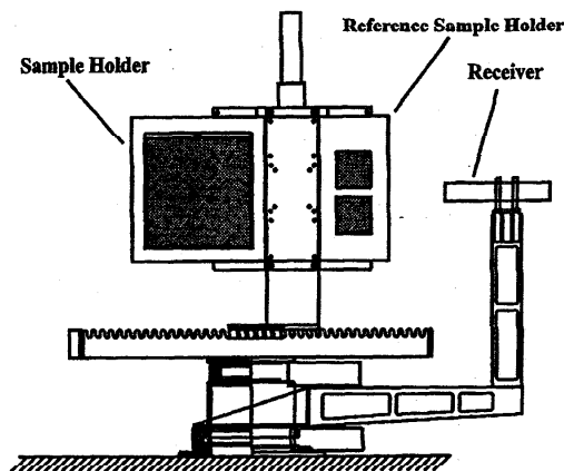
Fig. 2. Front view of the STARR goniometer.
