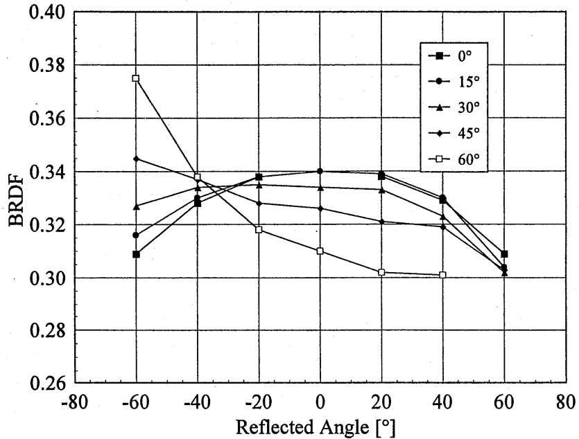
Figure 3.9. BRDF as a function of reflected angle at 632.8 nm for a PTFE plaque at the indicated incident angles. The relative expanded uncertainties of the BRDF, less than 0.2 percent, are within the sizes of the symbols.
