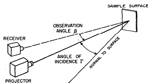
FIGURE 14. Diagram of apparatus used in retroreflectance measurements.
