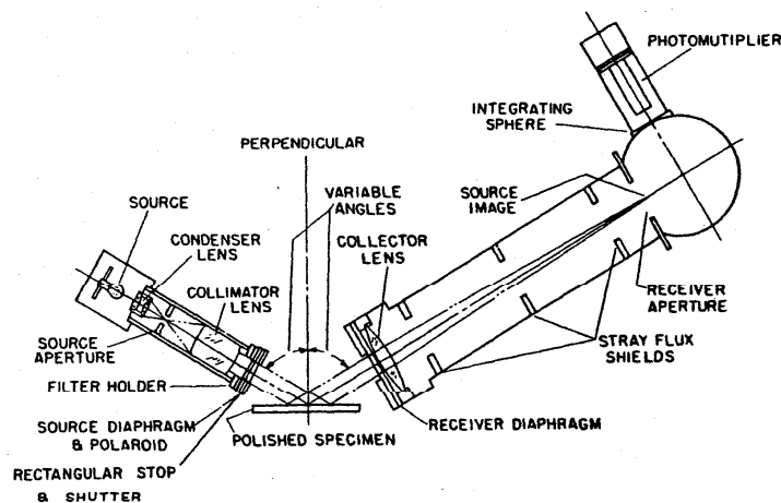
FIGURE 7. NBS-Gaertner goniophotometer.
