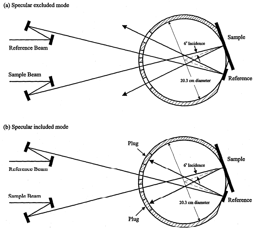
Figure 4.1. Top view of the Integrating Sphere Assembly of the Perkin-Elmer Lambda 19 transfer spectrophotometer configured for reflectance operating in the specular excluded (a) and specular included (b) modes.
