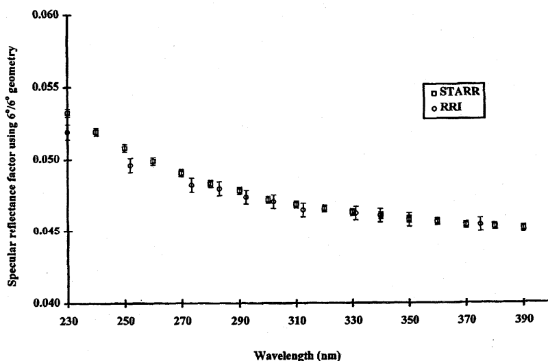
Fig. 6. Specular reflectance factor of GL-2 black glass using 6°/6° geometry as measured by STARR and by RRI.
