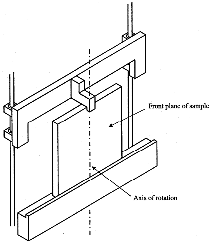
Figure 3.6. Sample mount of the STARR goniometer.
