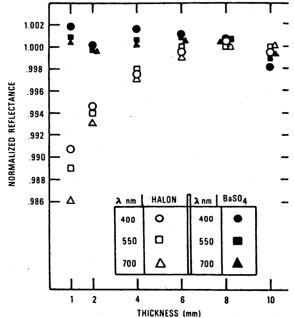
FIGURE 4. Reflectance of wall coatings as function of thickness. (Normalized to give a reflectance of approximately 1 for thick samples.)
