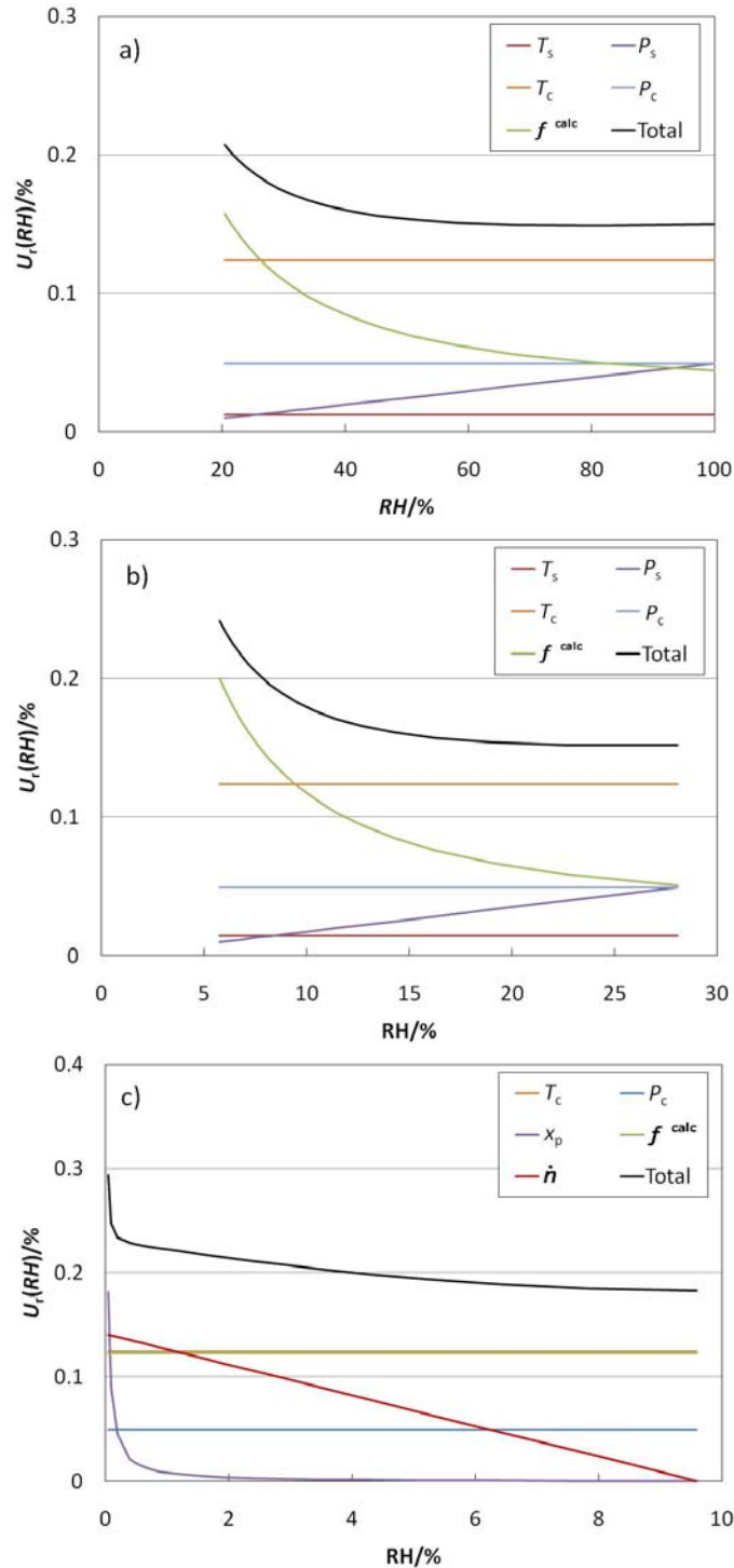
Figure 15. Total expanded relative uncertainty U_r(RH) for the relative humidity calibrations using humid gas generated by the HHG to an environment of temperature T_c = 20\text{ }^\circ\text{C} and pressure P_c = 100\text{ kPa} ; here, U_r(RH) includes the uncertainty for the calibration of the hygrometer's external temperature probe. In plots a) and b), the generator is used in 2-P mode, and the saturator temperature is a) 20\text{ }^\circ\text{C} and b) 1\text{ }^\circ\text{C} ; the relative humidity is varied by changing the saturator pressure. In c) the generator is used in divided-flow mode.
