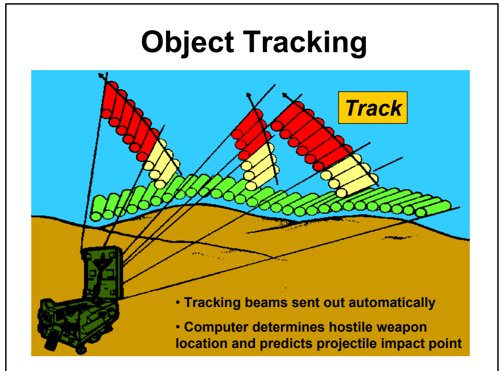
Figure 4-7. Object Tracking
