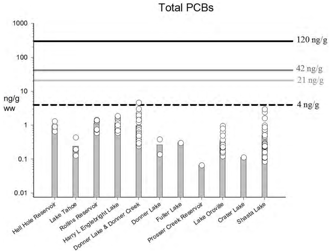
Figure 6.6.2 Total PCBs
