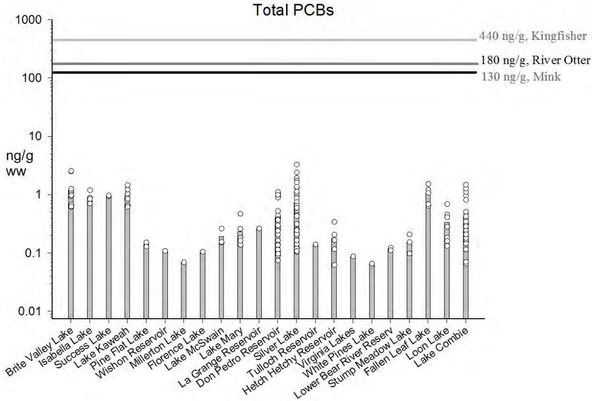
Figure 8.4.1 Total PCBs
