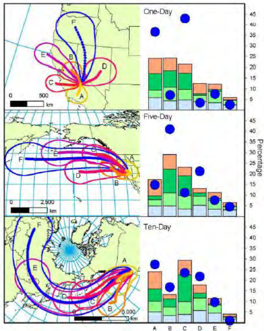
Figure 4. WACAP 1, 5, and 10 day air mass back trajectories for SEKI [1].
