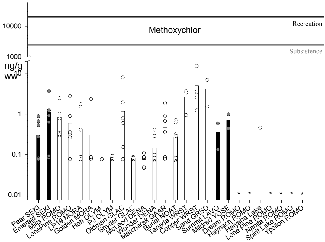
Figure 5-12: Methoxychlor
