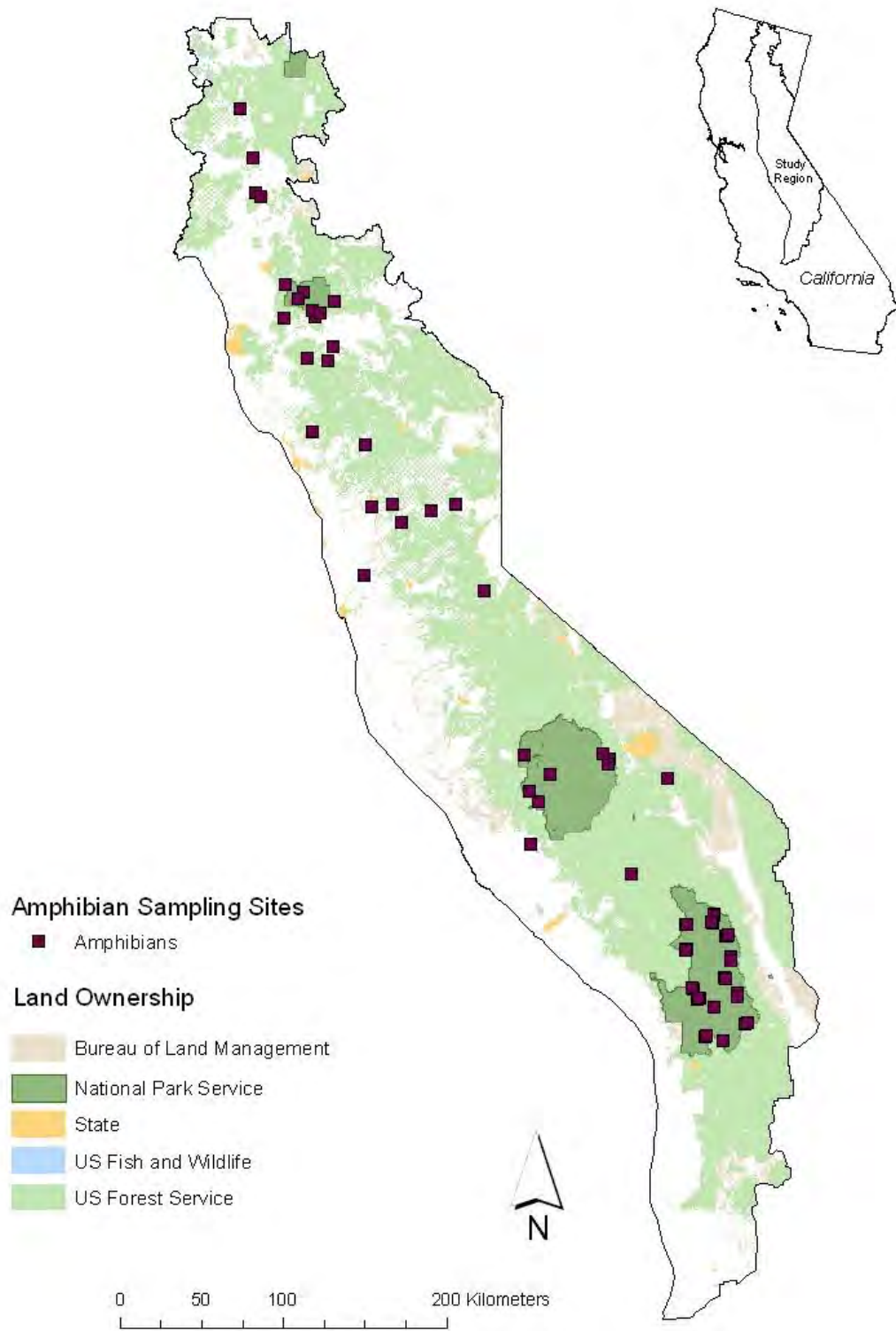
Figure 44. Amphibian sampling sites (1997–2005).
