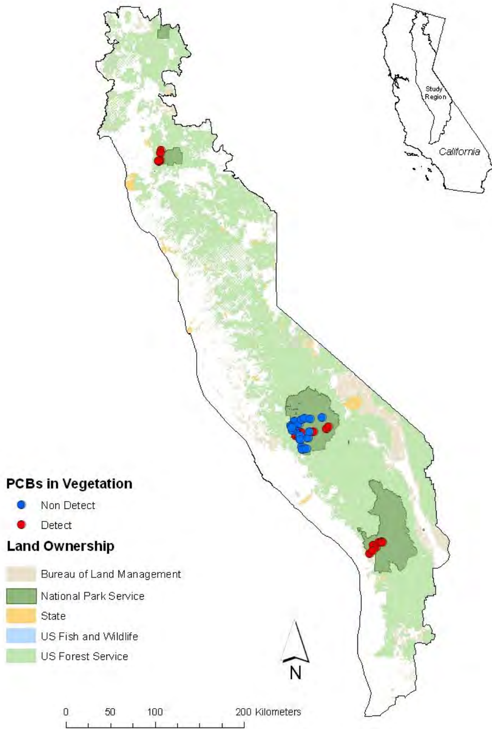
Figure 41. Polychlorinated Biphenyls (PCBs) detection in vegetation (2002–2009).
