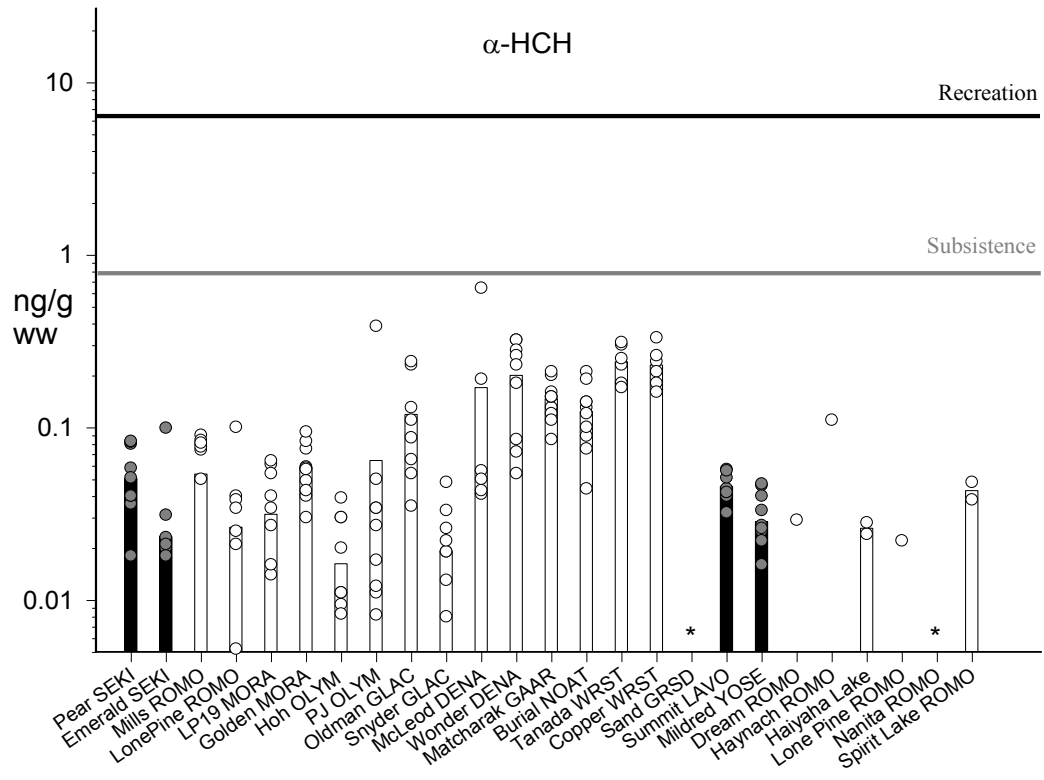
Figure 5.3. Median α-HCH
