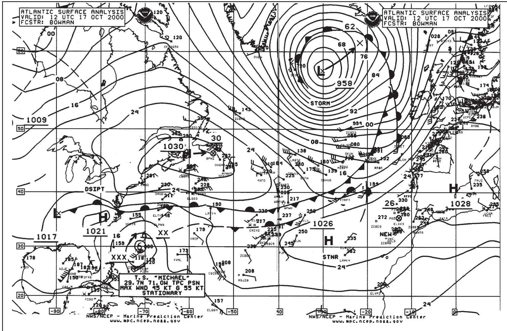
Figure 5. MPC North Atlantic Surface Analysis chart valid 1200 UTC October 17, 2000.
