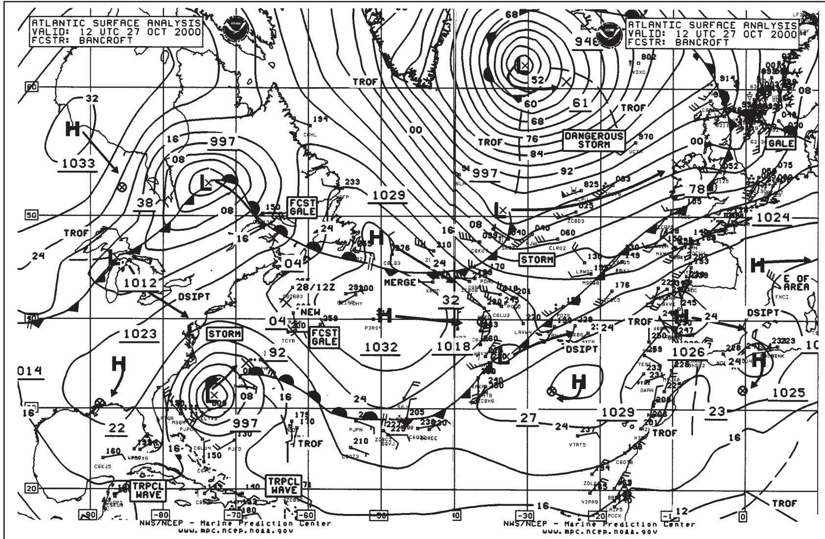
Figure 8. MPC North Atlantic Surface Analysis chart valid 1200 UTC October 27, 2000.
