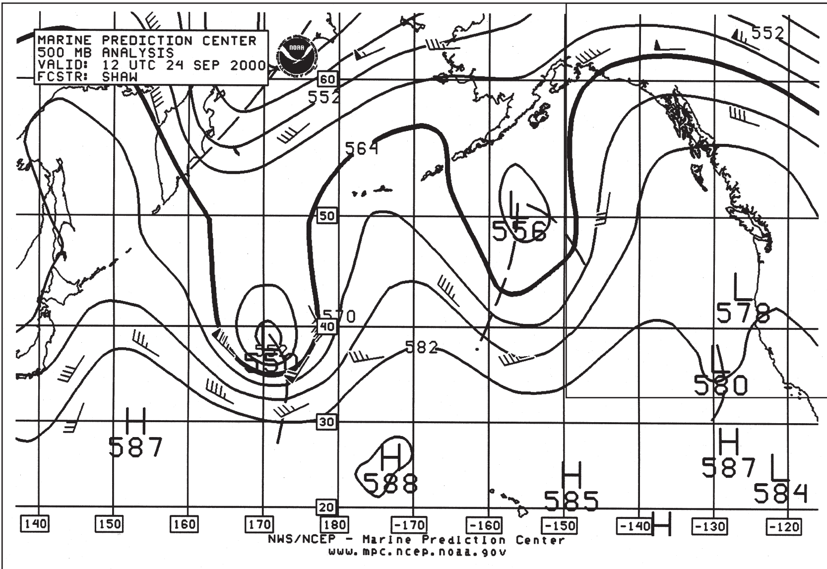
Figure 2. MPC 500-Mb Analysis of North Pacific valid at 1200 UTC September 24, 2000.
