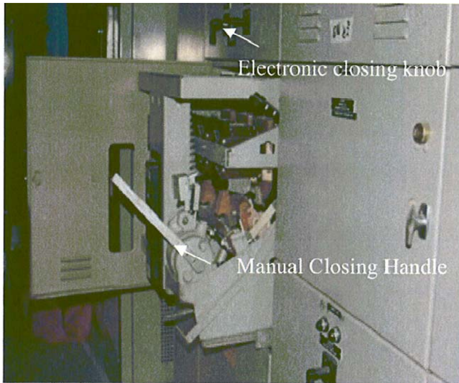
Figure 2-9: Racked Out Air Breaker
