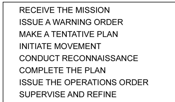
Figure 2-3. Troop-leading procedures.
