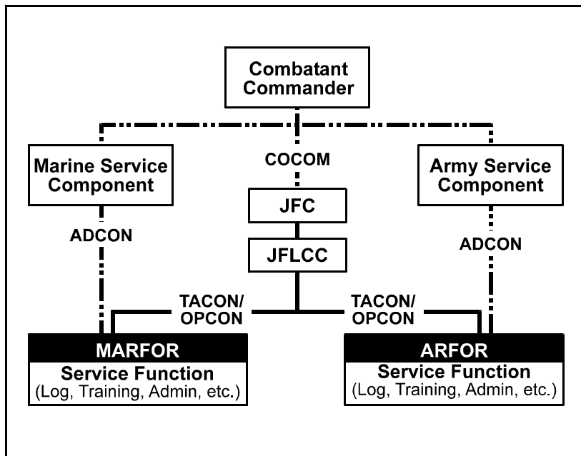
Figure II-2. Service Functions
