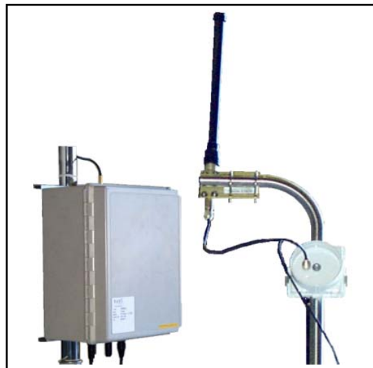
Figure C-10. RF Relay
