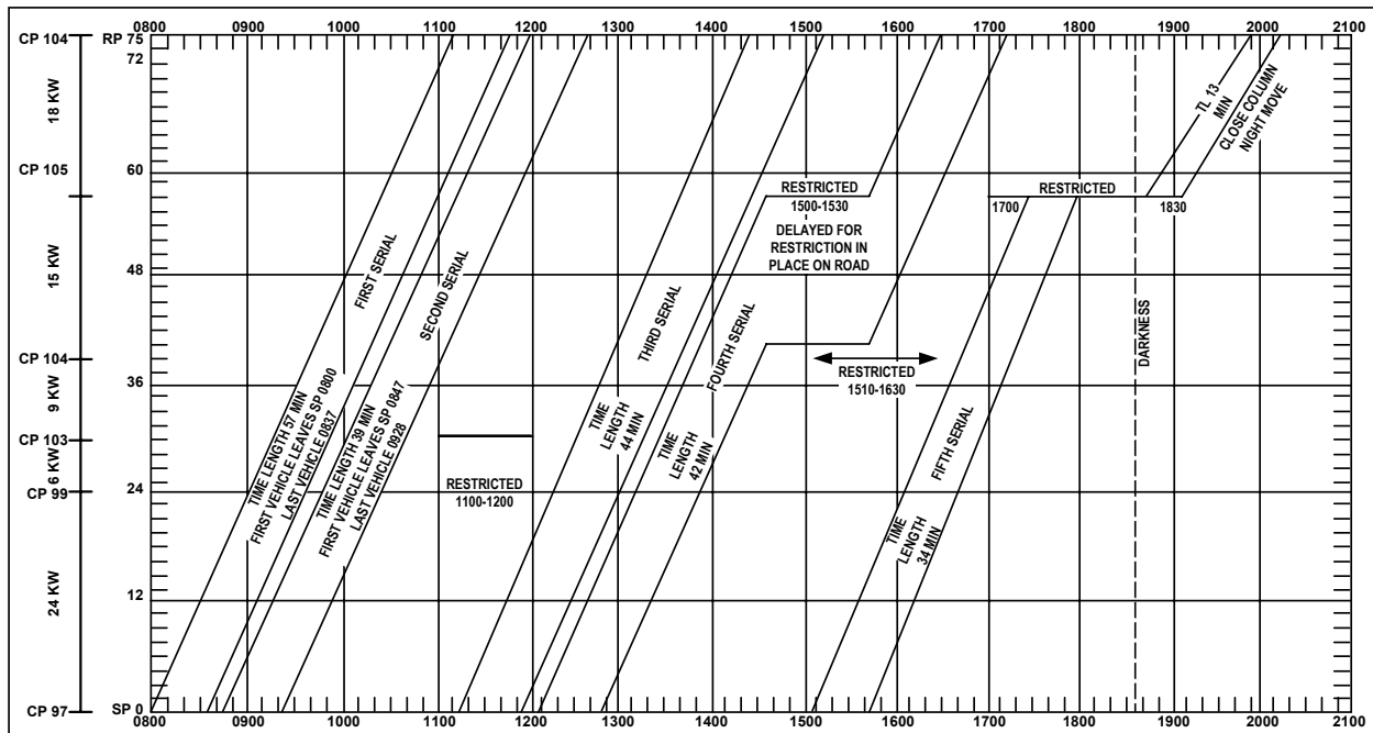
Figure G-8. Road Movement Graph for Five Serials
