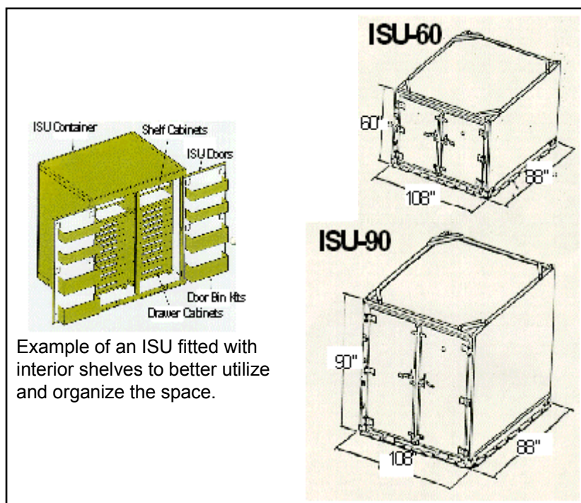
Figure J-15. ISU-60, -90, and -96
