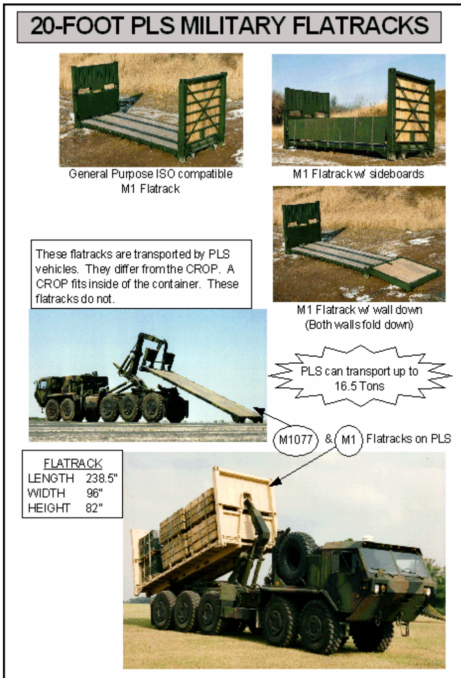
Figure J-16. 20-Foot PLS Flatracks
