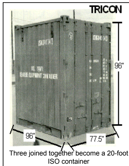
Figure J-14. TRICON
