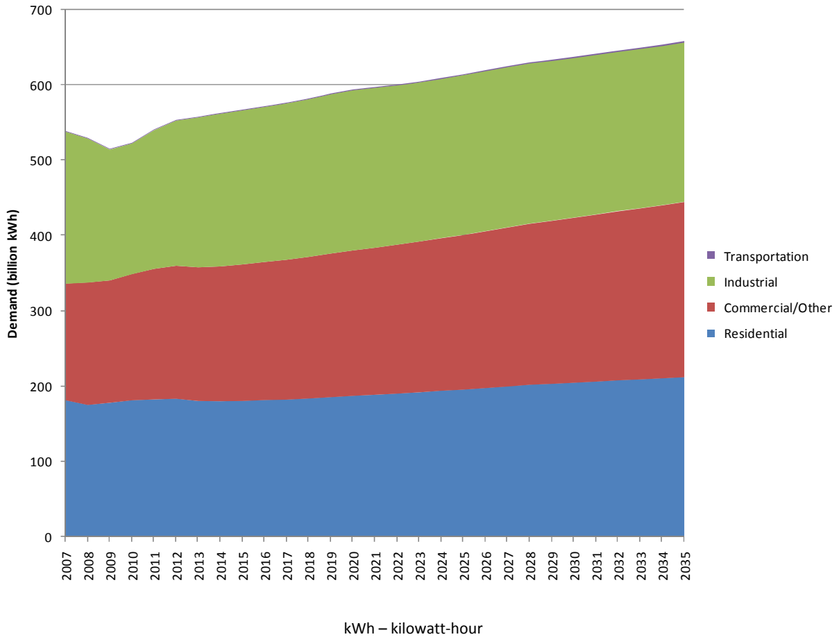
Figure 52. East Central Area Reliability Coordination Agreement projected electricity demand, 2007-2035. Data: EIA (December 2009).*
