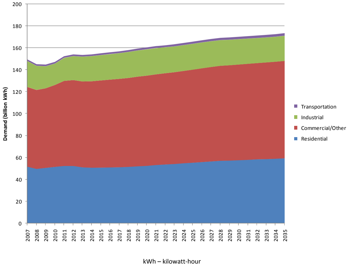
Figure 57. Northeast Power Coordinating Council/New York projected electricity demand, 2007-2035. Data: EIA (December 2009).*
