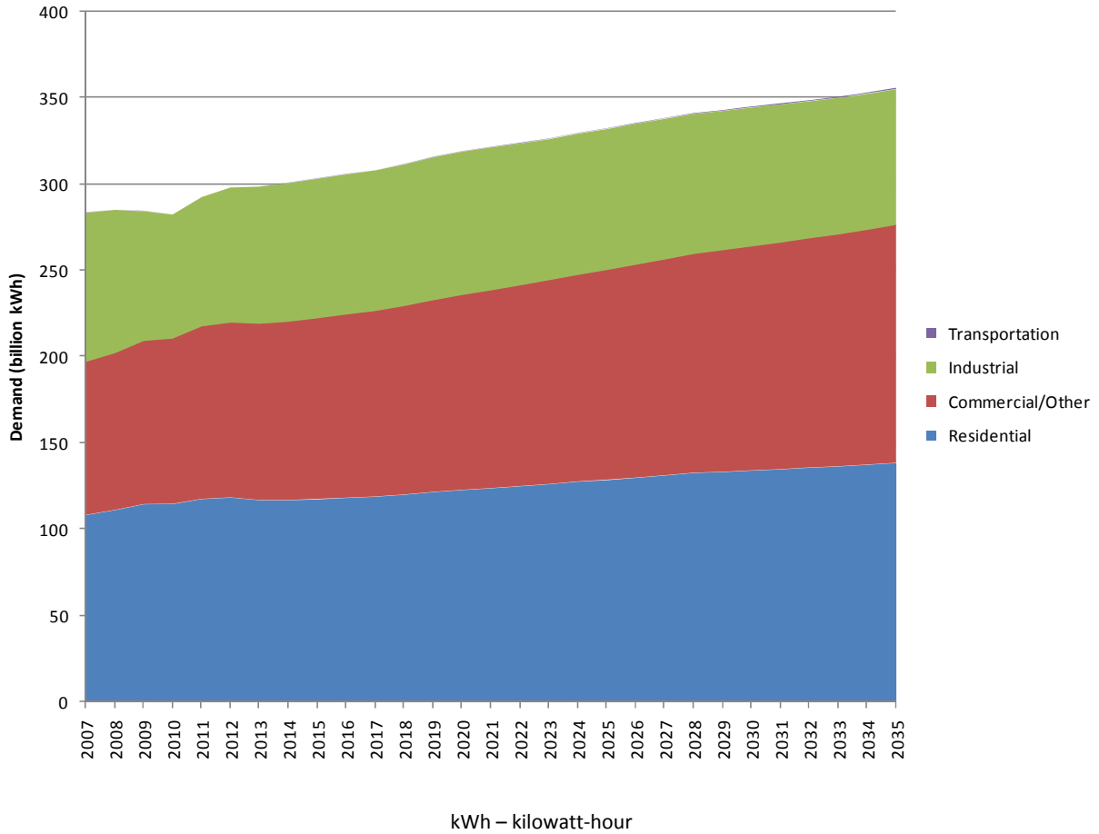
Figure 53. Electric Reliability Council of Texas projected electricity demand, 2007-2035. Data: EIA (December 2009).*
