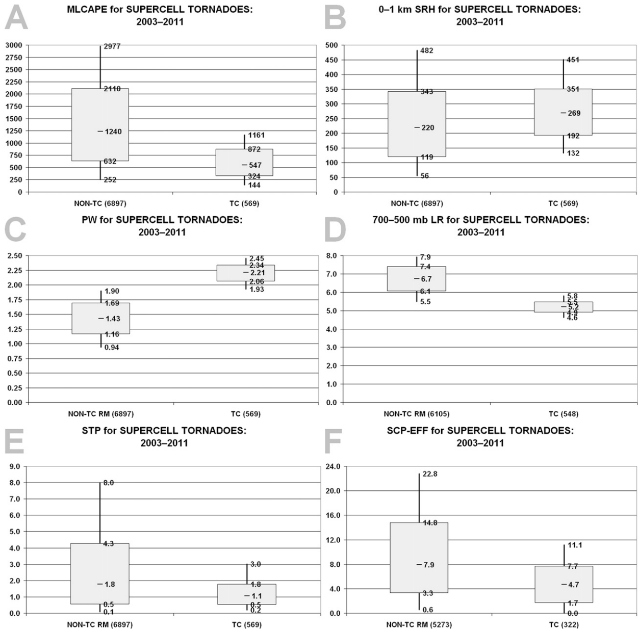
FIG. 8. As in Fig. 7, but for the following parameters in TC and non-TC tornadic supercell datasets: (a) MLCAPE ( \text{J kg}^{-1} ), (b) 0–1-km AGL SRH ( \text{m}^2 \text{s}^{-2} ), (c) precipitable water (in.), (d) 700–500-hPa lapse rate ( ^{\circ}\text{C km}^{-1} ), (e) significant tornado parameter (fixed layer), and (f) supercell composite parameter (effective layer).
