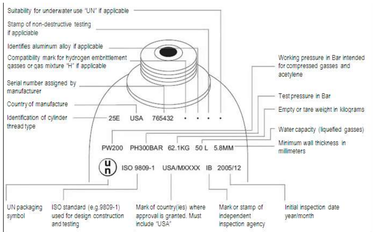
Figure A14.3. Sample of UN Specification Marking for UN Pressure Receptacles.
