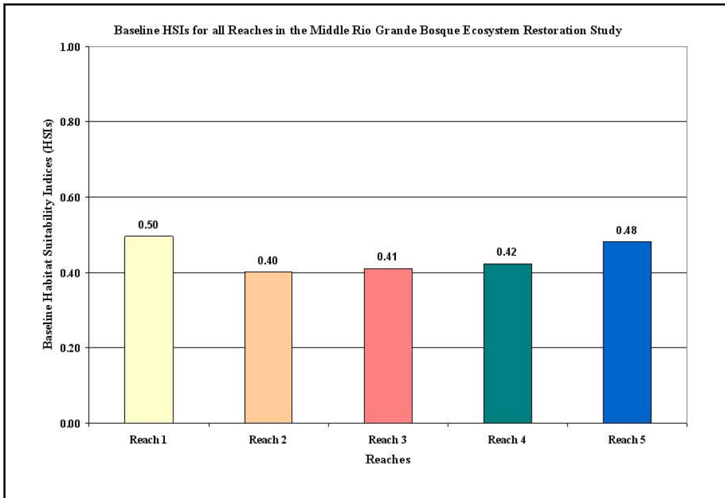
Figure 36. Baseline HSI results for the MRGBER study based on the bosque community index model.
