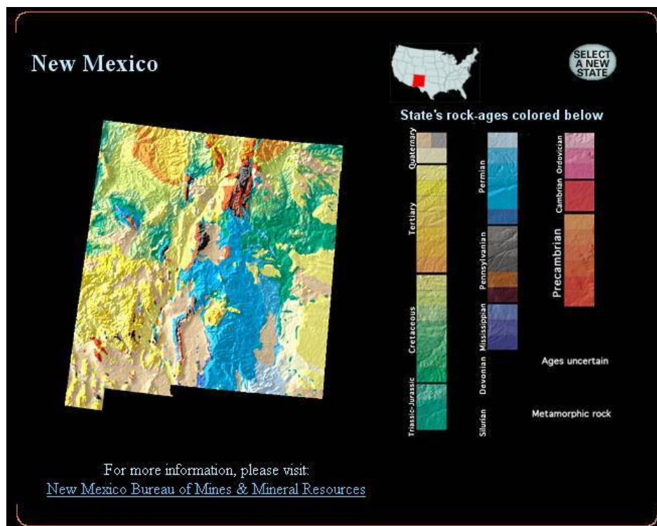
Figure 15. Topography and underlying geology for the state of New Mexico. 1
