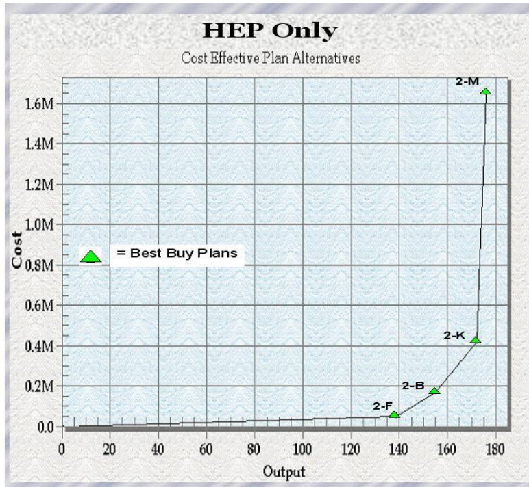
Figure 51. Cost effective analysis results (graphical depiction) for Reach 2 plans.
