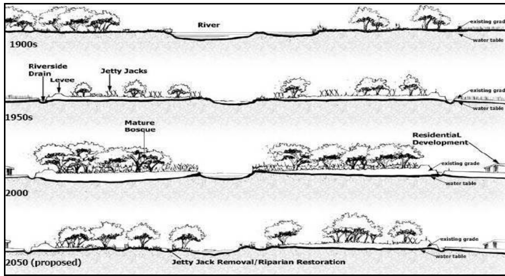
Figure 6. Flood protection projects (e.g., levees, riverside drains and jetty jacks) have reduced the Middle Rio Grande's original floodplain to fraction of its size in the study area (USACE 2003a).
