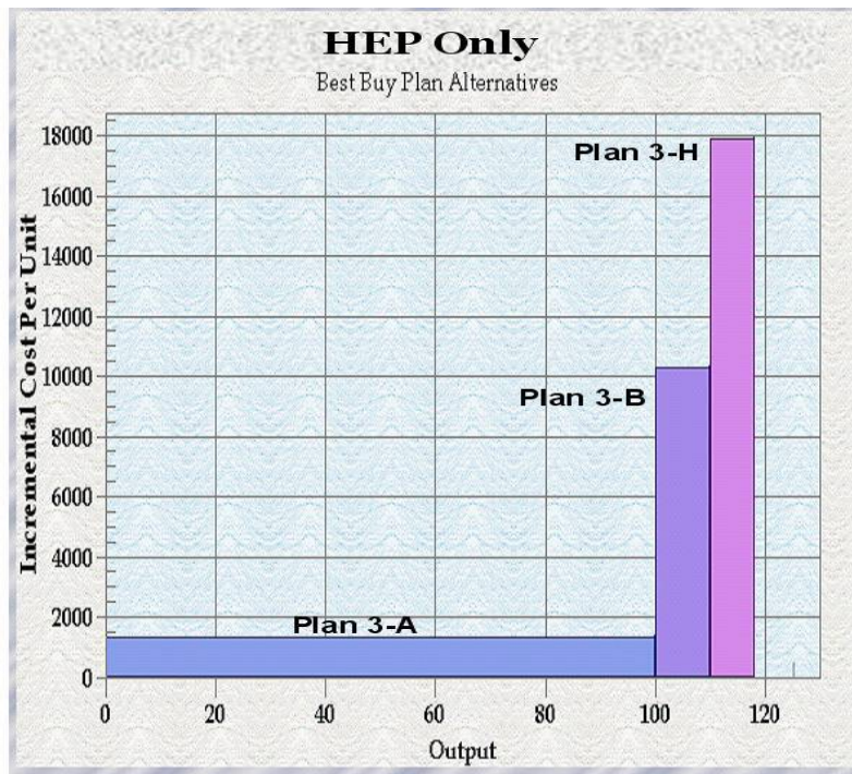
Figure 57. Incremental cost analysis results (graphical depiction) for the Reach 3 plans.
