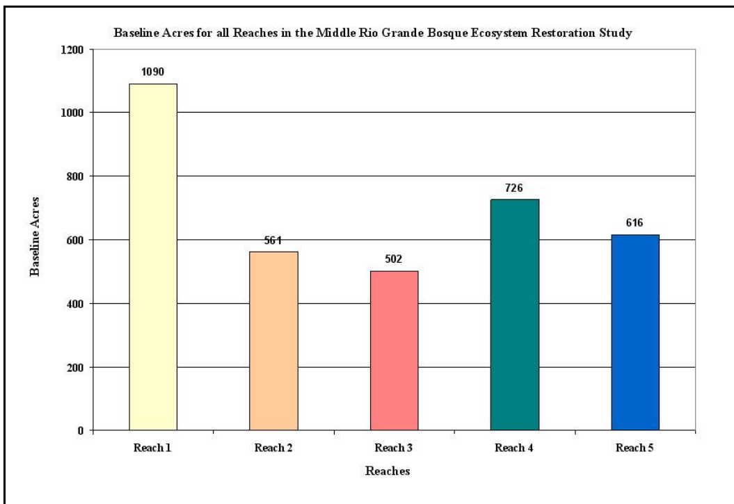
Figure 37. Baseline acre distributions for the MRGBER study based on the bosque community index model.
