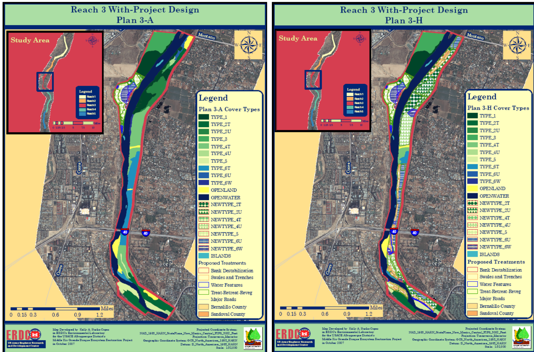
Figure 46. "Maximum" and "Minimum" plans for Reach 3 in the MRGBER study.
