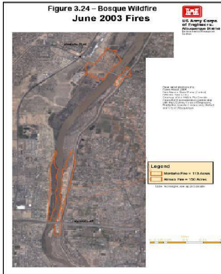
Figure 27. Location of 2003 bosque fires (map taken from USACE 2007 ).
