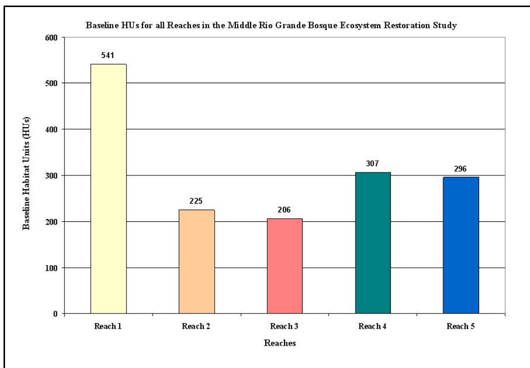
Figure 38. Baseline HU results for the MRGBER study based on the bosque community index model.
