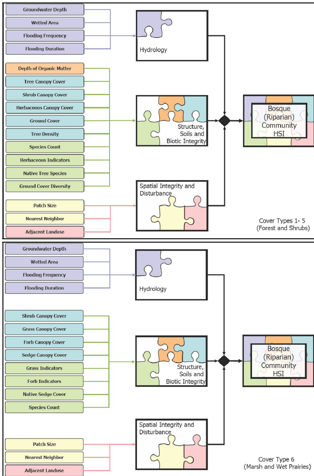
Figure 31. Flow diagram depicting combinations of model components and variables to form the Bosque community index model in the MRGBER study. There are two versions of the model depending on the cover types being evaluated. Types I-V use the upper diagram, and Type VI uses the lower diagram.
