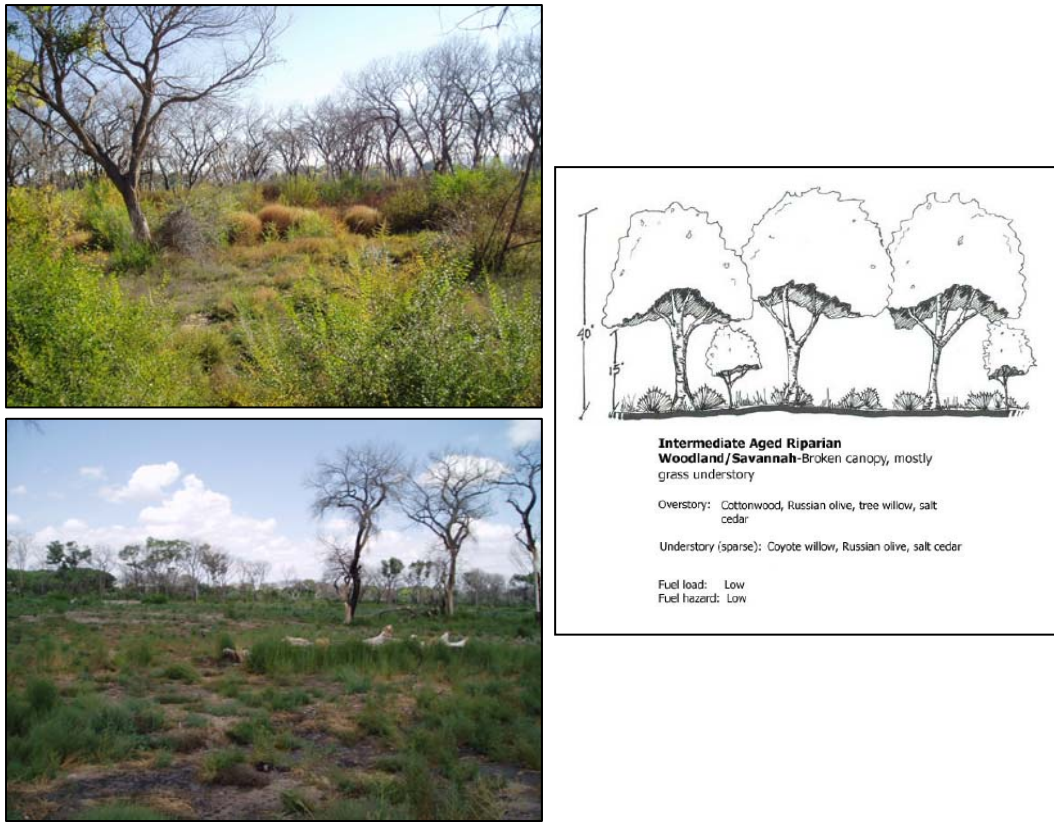
Figure 23. Classic examples of Type IV (Intermediate-aged Riparian Woodland/Savannahs) vegetation in the study area.
