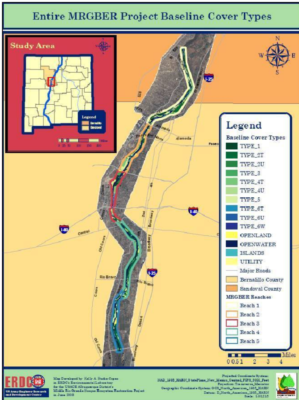
Figure 28. Baseline cover type map for the project study area.
