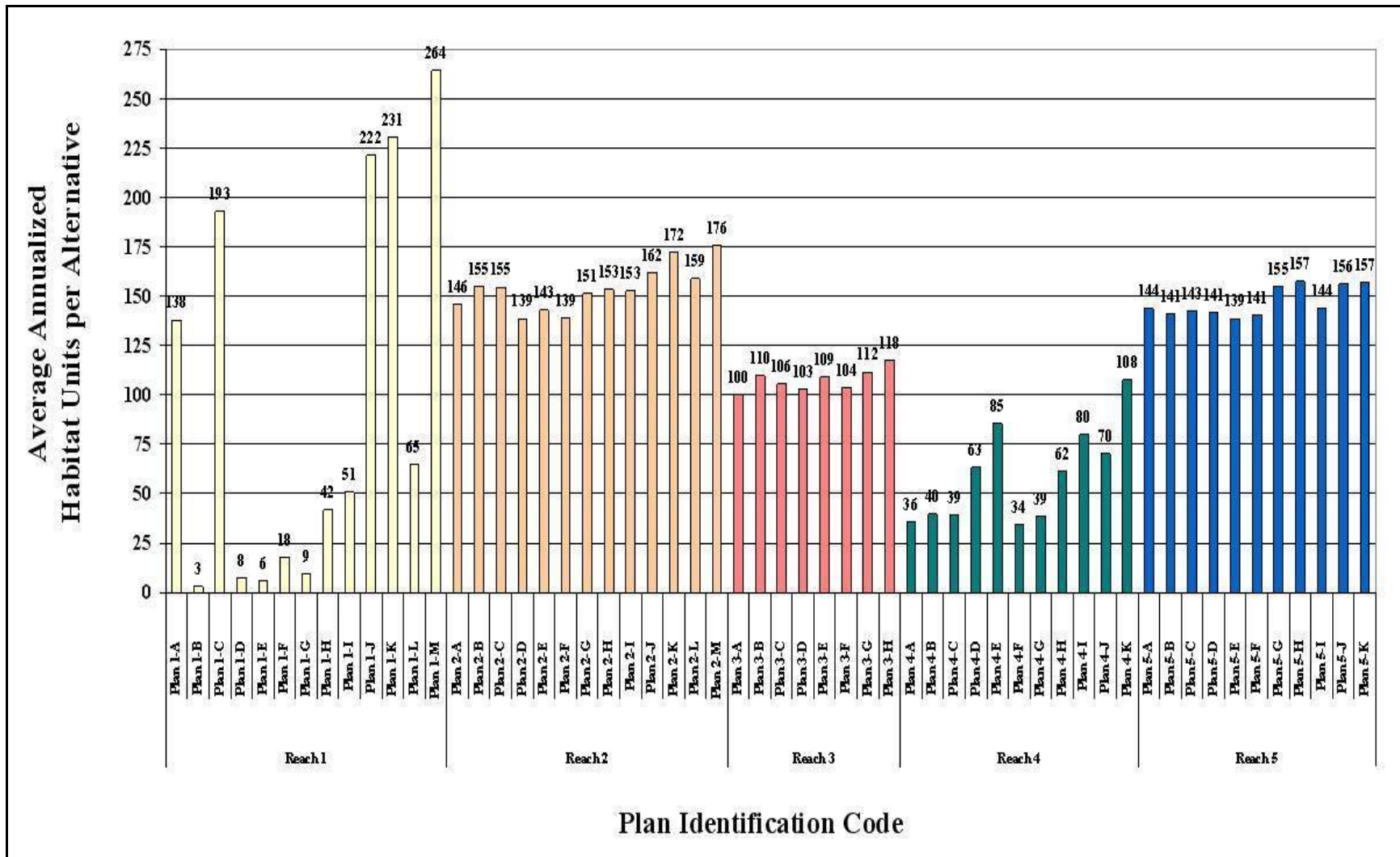
Figure 49. Final results of the MRGBER study HEP analysis.
