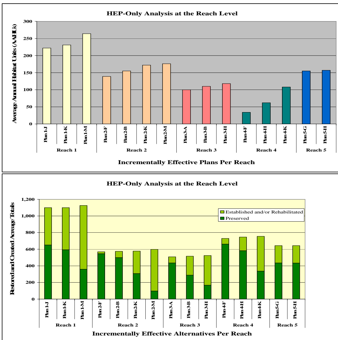
Figure 60. Comparison of Best Buy solutions for the MRGBER study on a reach-by-reach basis (ecosystem outputs and established/preserved acreages).
