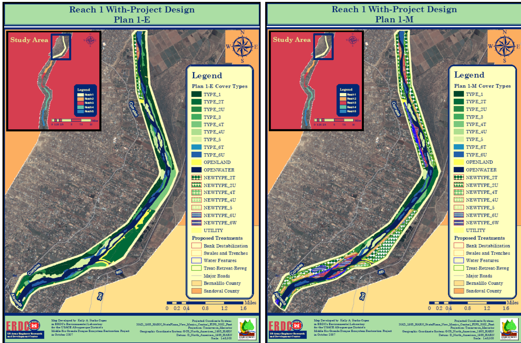
Figure 44. "Maximum" and "Minimum" plans for Reach 1 in the MRGBER study.
