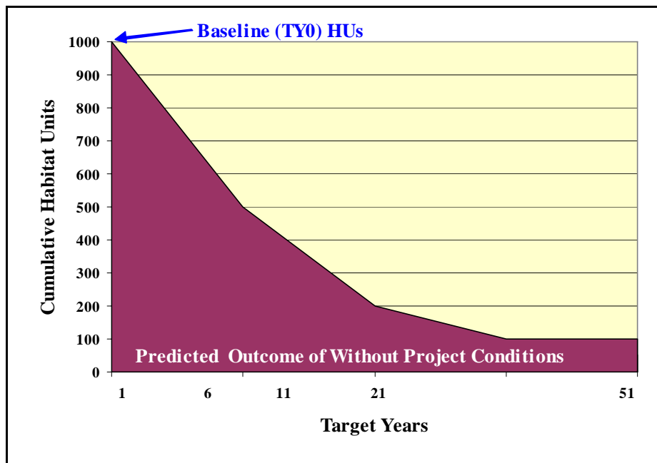
Figure 34. Example of cumulative HU availability under a Without-project scenario
