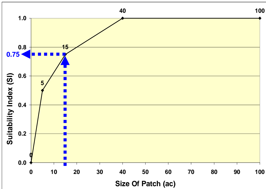
Figure 33. Example Suitability Index (SI) curve.
