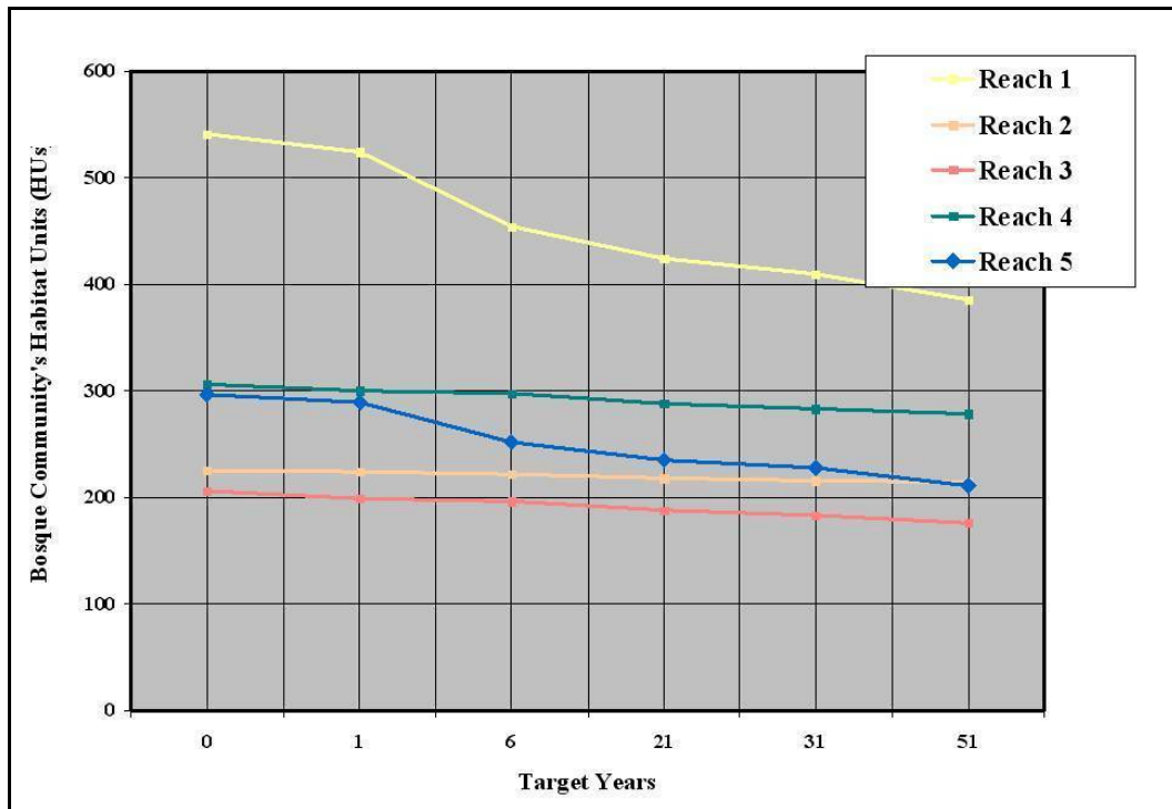
Figure 43. Cumulative changes in HUs under the WOP scenario.
