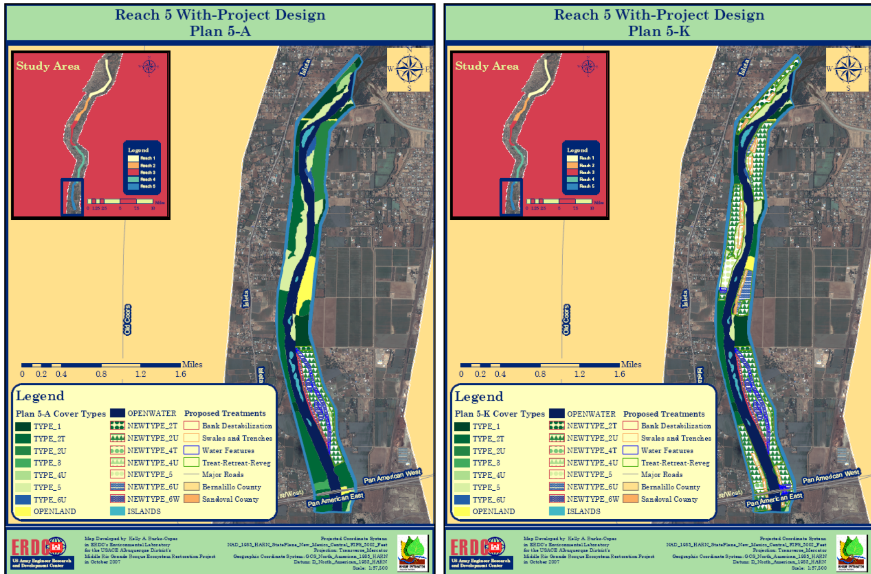
Figure 48. "Maximum" and "Minimum" plans for Reach 5 in the MRGBER study.
