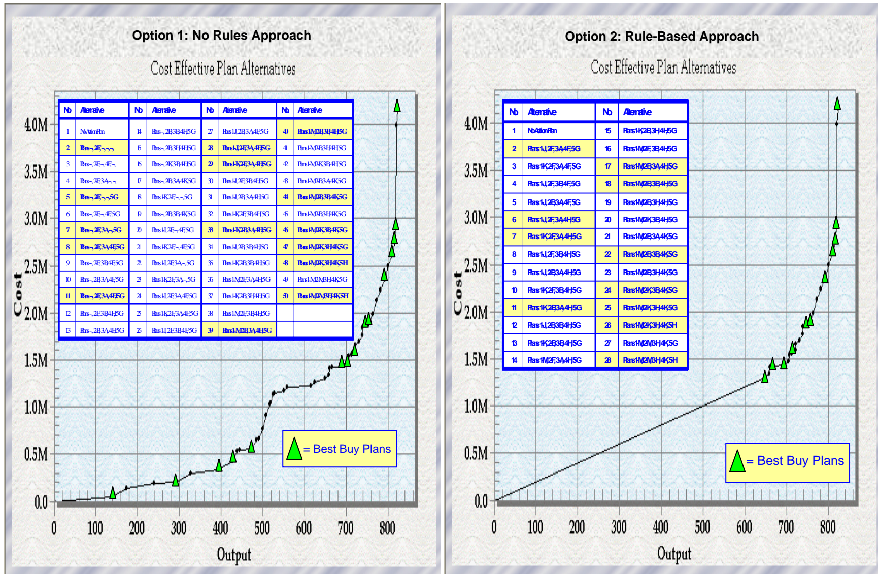
Figure 61. Graphical comparison of the cost effective results for the entire MRGBER project under the two options (the “No rule” option is on the left and the “Rule-based” option is on the right).
