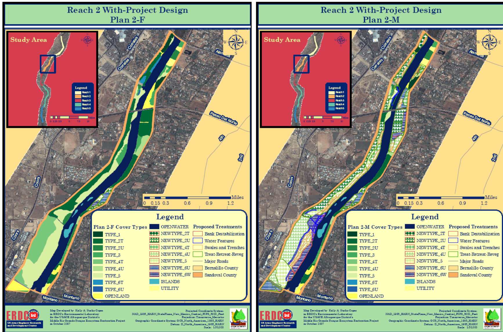
Figure 45. "Maximum" and "Minimum" plans for Reach 2 in the MRGBER study.
