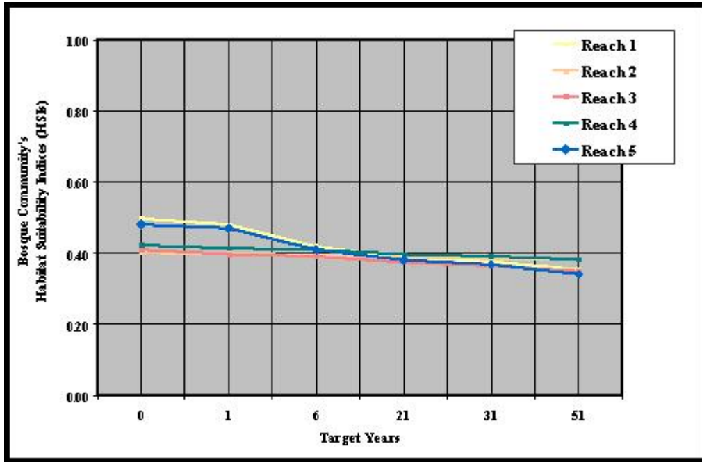
Figure 42. Cumulative changes in HSI under the WOP scenario.
