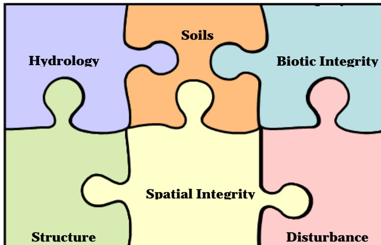
Figure 30. Within the conceptual modeling building framework, the various model components (color-coded for organization purposes) are pieced together to capture the essence of community functionality using the ecosystem puzzle analogy.
