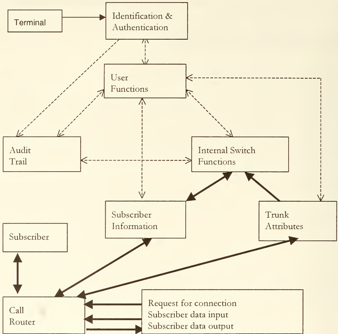
Figure 2. PBX Functional Architecture
