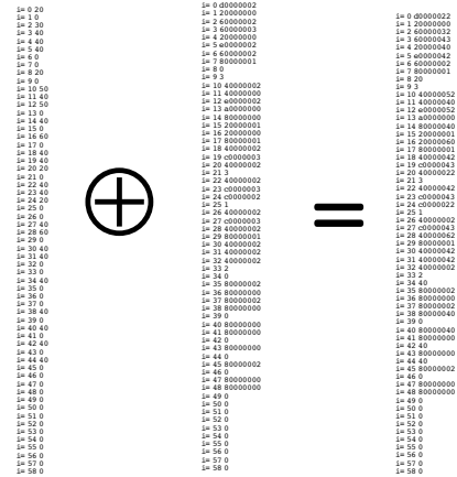
Figure 1: Finding good disturbance vector (I)
