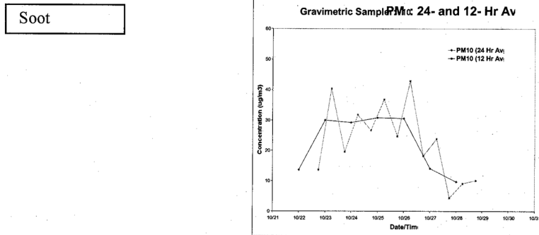
Figure 3. Concentrations of Black Carbon (Soot) and \text{PM}_{10} Mass Measured at NYU Downtown Hospital.
