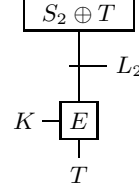
Fig. 9. Illustration of adversary's forgery attempt. We see that T = \text{OMAC1}'_K(S_2 \oplus T) .
