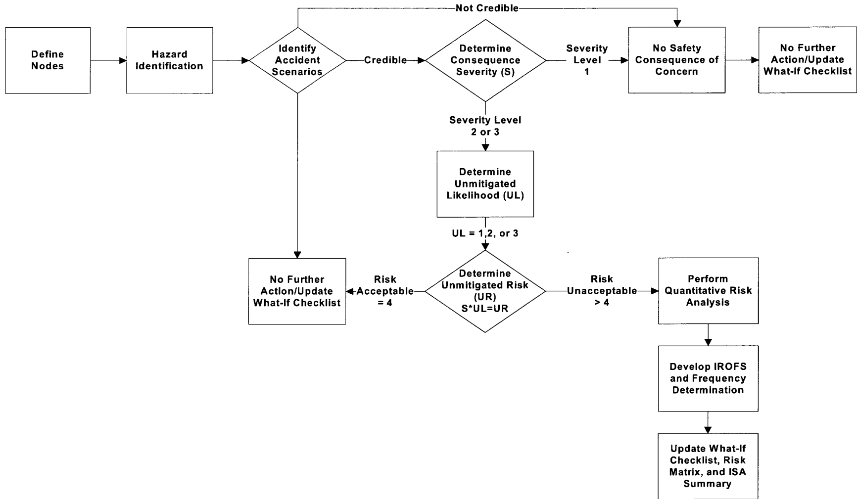
Figure 3-1. Integrated Safety Analysis Process Flow Diagram.
