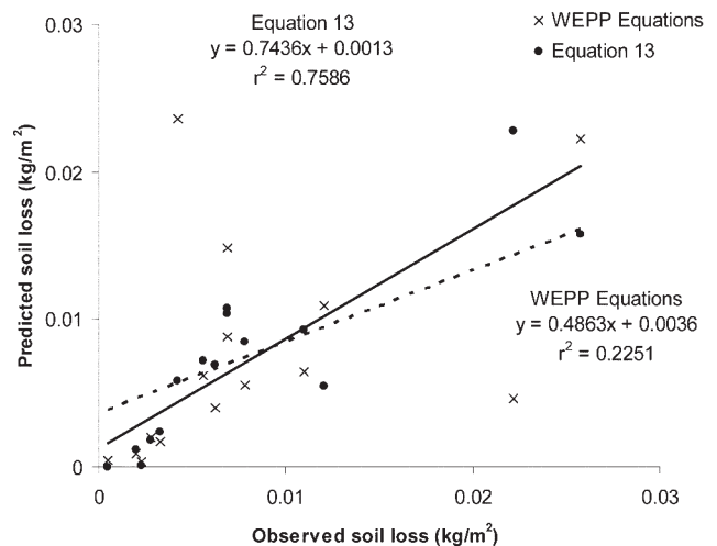
Fig. 6. Comparison of soil loss predictions from the new splash and sheet erosion equation and those from the Water Erosion Prediction Project (WEPP) model based on rainfall simulation plot data ( n = 15 ), suggesting that the new equation provided better predictions.
