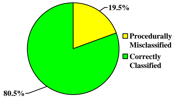
Figure 2 Procedural Misclassifications
