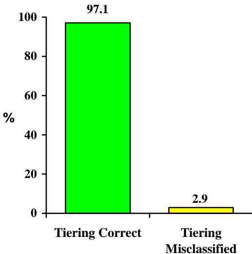
Figure 3 Verified Classifications
