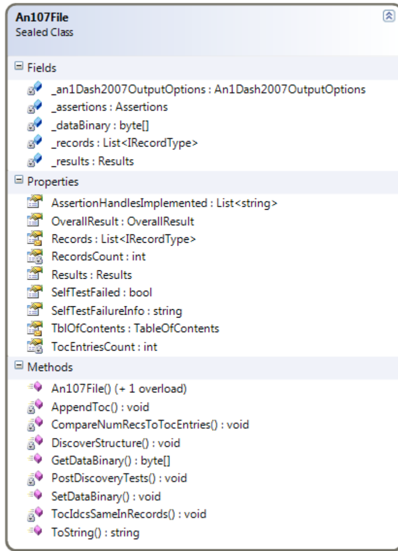
Figure A-1: Class Diagram for the An107 File Class
