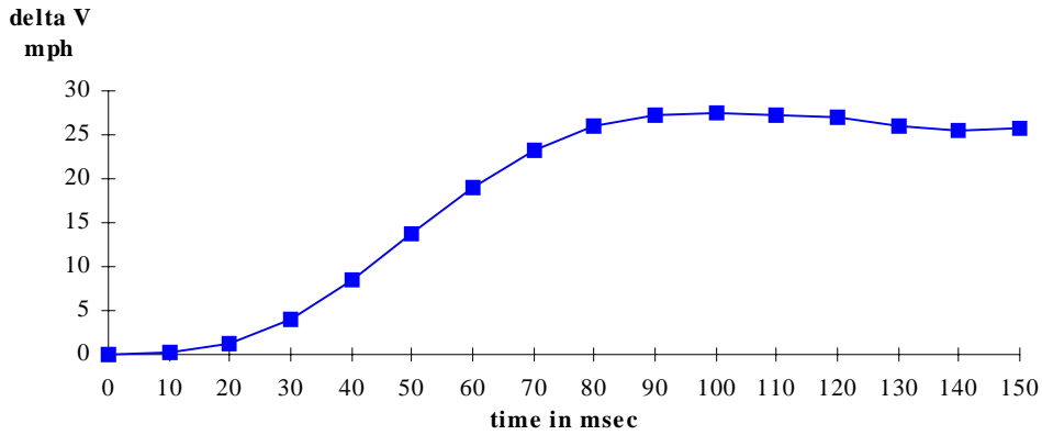
Figure 2: Post-impact \Delta V vs. time
