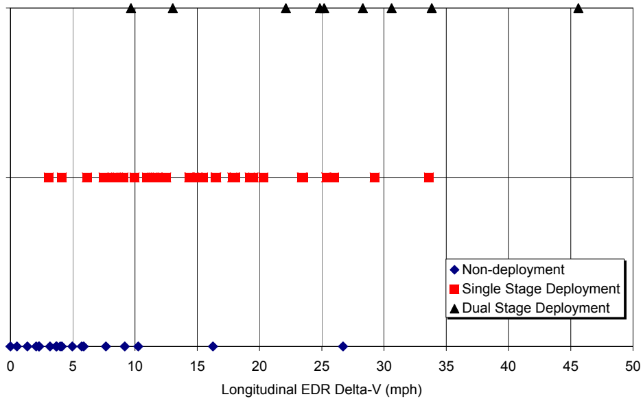
Figure 13. Distribution of Driver Air bag Dual-Stage, Single-Stage, and Non-deployments versus Delta V
