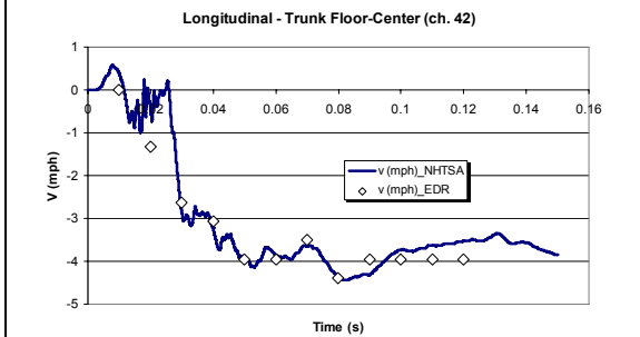
Figure 28. NHTSA Test 5260- 2005 Saturn Ion – Side Impact (with no EDR time shift)
