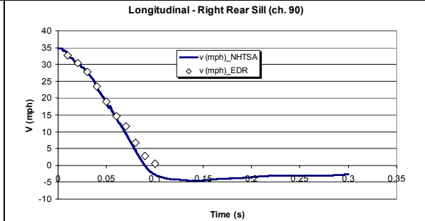
Figure 27. NHTSA Test 5324- 2005 Pontiac Montana (with no EDR time shift)
