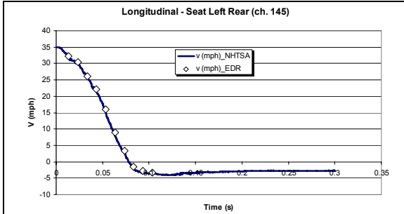
Figure 24. NHTSA Test 5310- 2005 Buick Rendezvous (with EDR time shift of -.0035s)
