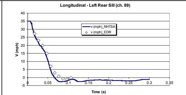
Figure 25. NHTSA Test 5282- 2005 Chevrolet Colorado (ext.cab) (with EDR time shift of -.007s)
