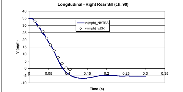
Figure 29. NHTSA Test 5318- 2005 Chevrolet Silverado (EDR time shift of -.005s)
