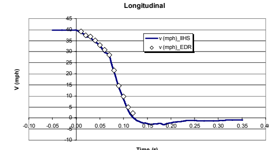
Figure 51. IIHS Test CEF0419- 2005 Saturn Ion (with no EDR time shift)
