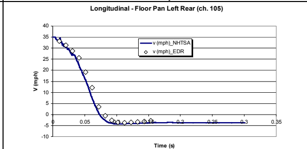
Figure 59. NHTSA Test 5160- 2005 Toyota Corolla (with no EDR time shift)
