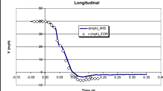
Figure 50. IIHS Test CF05003- 2004 Chevrolet Malibu – Pole Test (with no EDR time shift)
