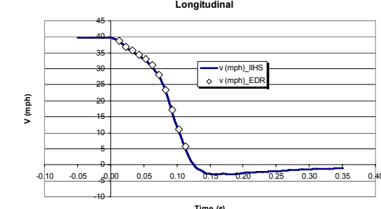
Figure 53. IIHS Test CEF0511- 2005 Buick LaCrosse (with no EDR time shift)
