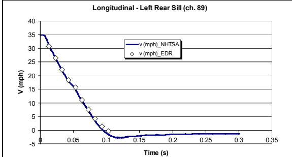
Figure 26. NHTSA Test 5265- 2005 Chevrolet Express (with EDR time shift of -.003s)
