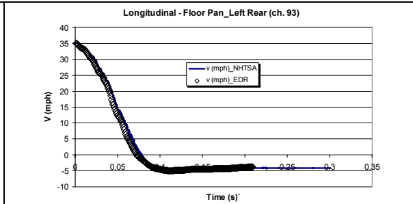
Figure 55. NHTSA Test 5263- 2005 Ford Freestyle (with no EDR time shift)
