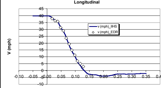
Figure 52. IIHS Test CEF0506- 2005 Chevrolet Colorado (with no EDR time shift)
