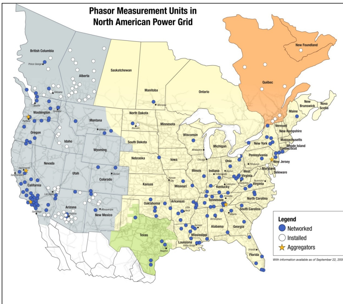
Figure A.30. Networked Phasor Measurement Units in the North American Power Grid 322
