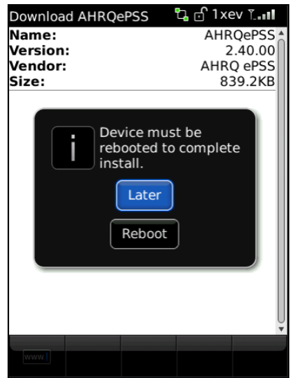
Figure 12: Reboot Screen
