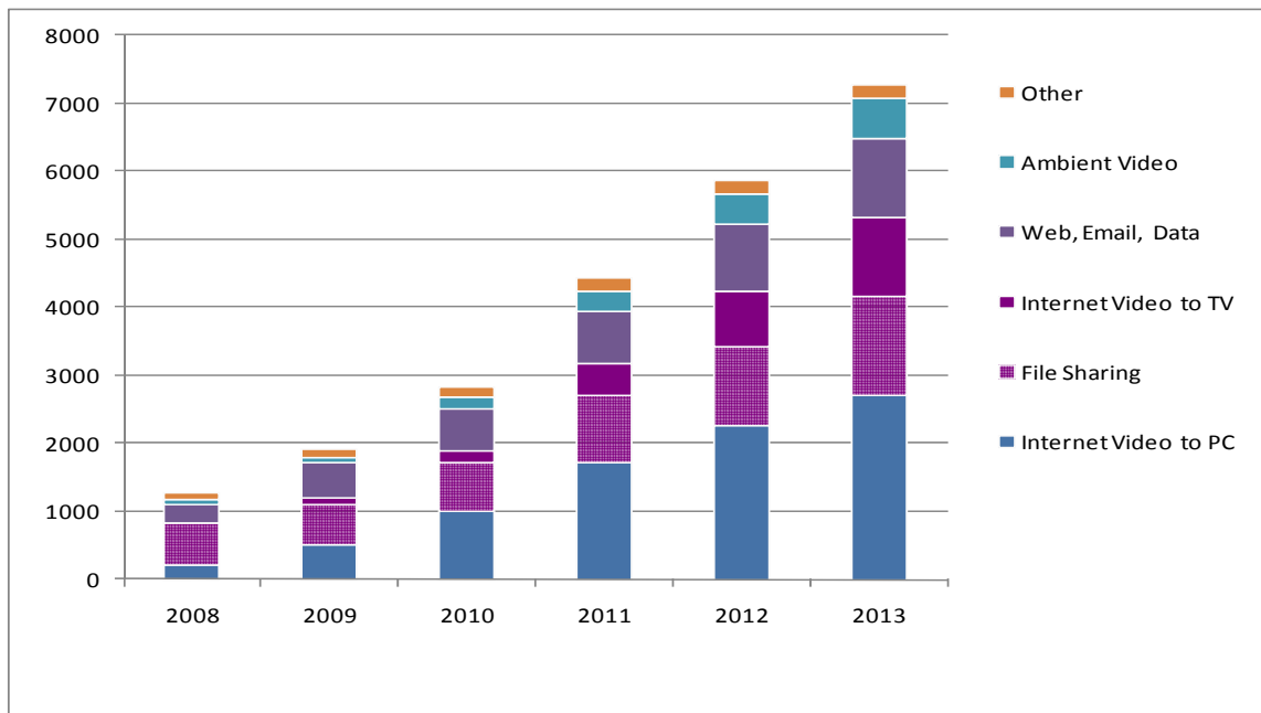
FIGURE 11: NORTH AMERICAN CONSUMER INTERNET TRAFFIC (Petabits/Month)
